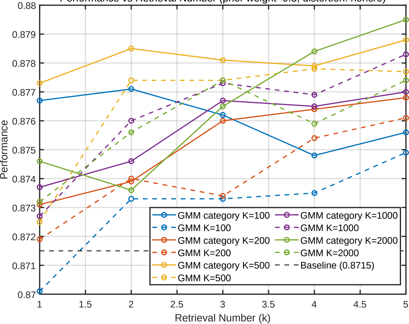
Performance vs Retrieval Number (prior weight=0.3, distortion: none/0)
