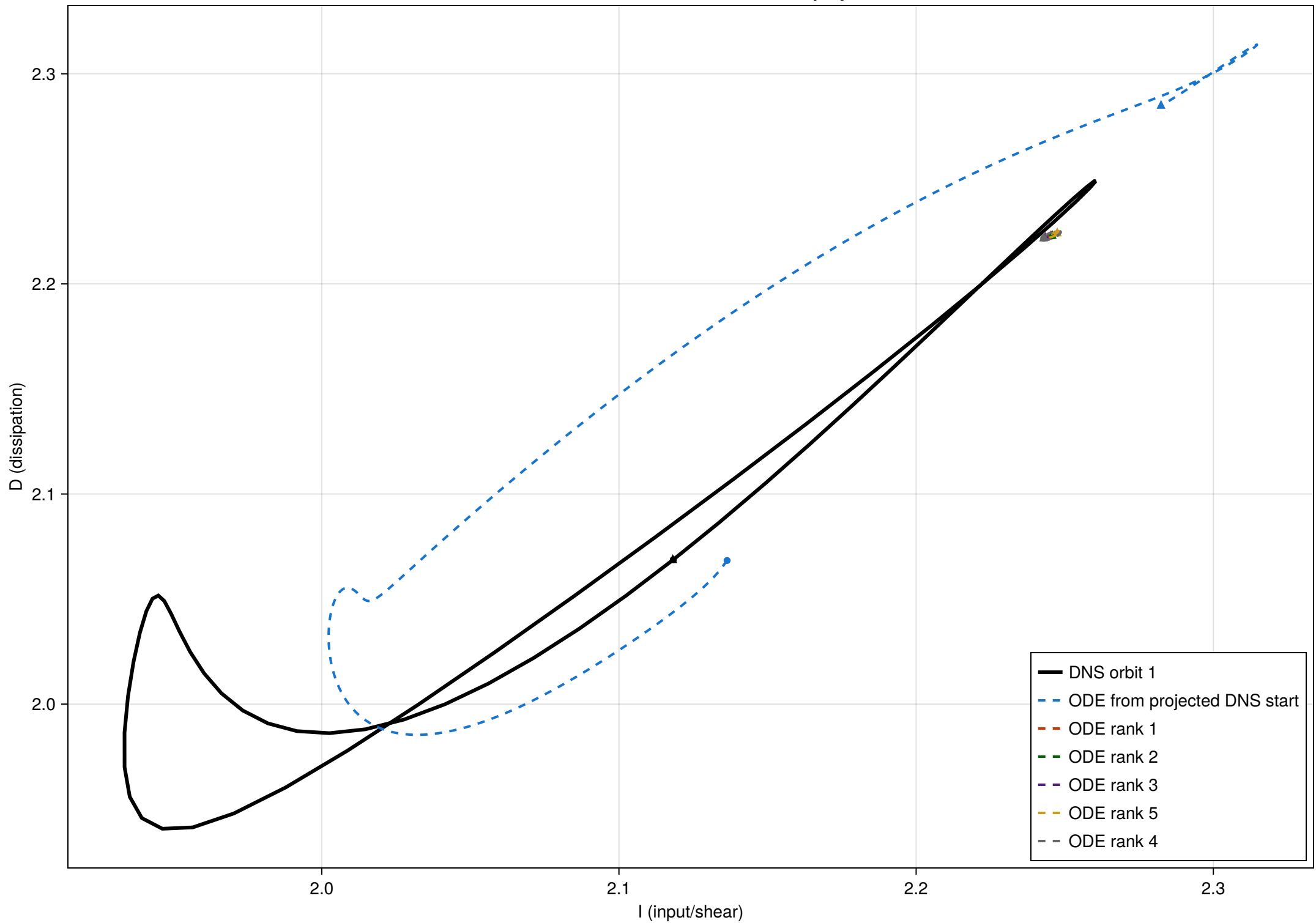
Gibson orbit 1: ODE candidates vs DNS projection
