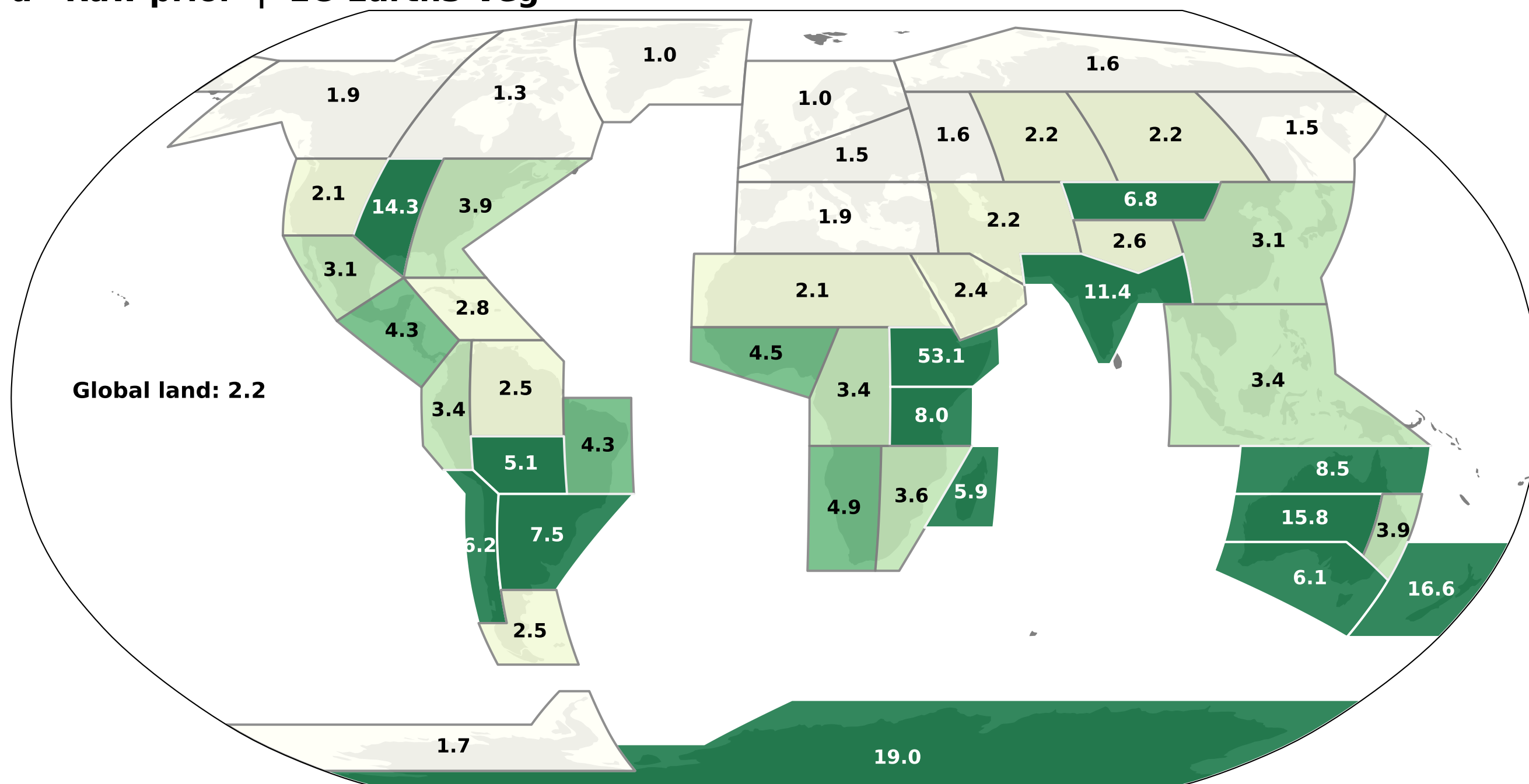
a Raw prior | EC-Earth3-Veg
