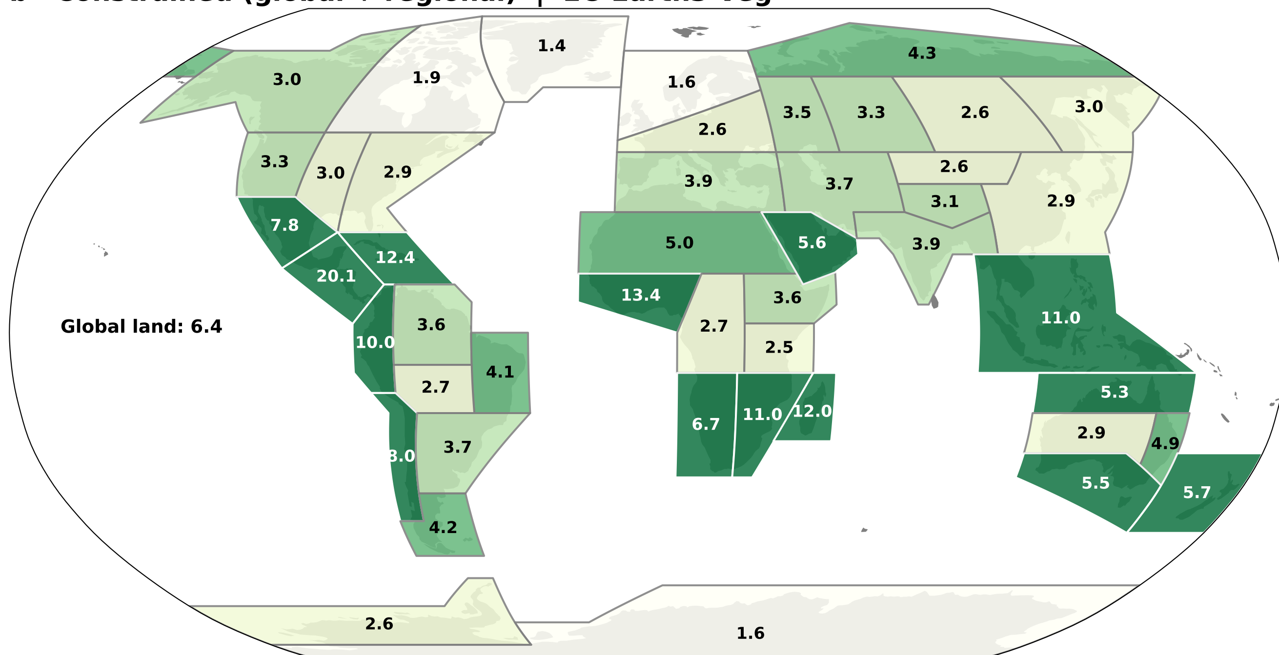
b Constrained (global + regional) | EC-Earth3-Veg
