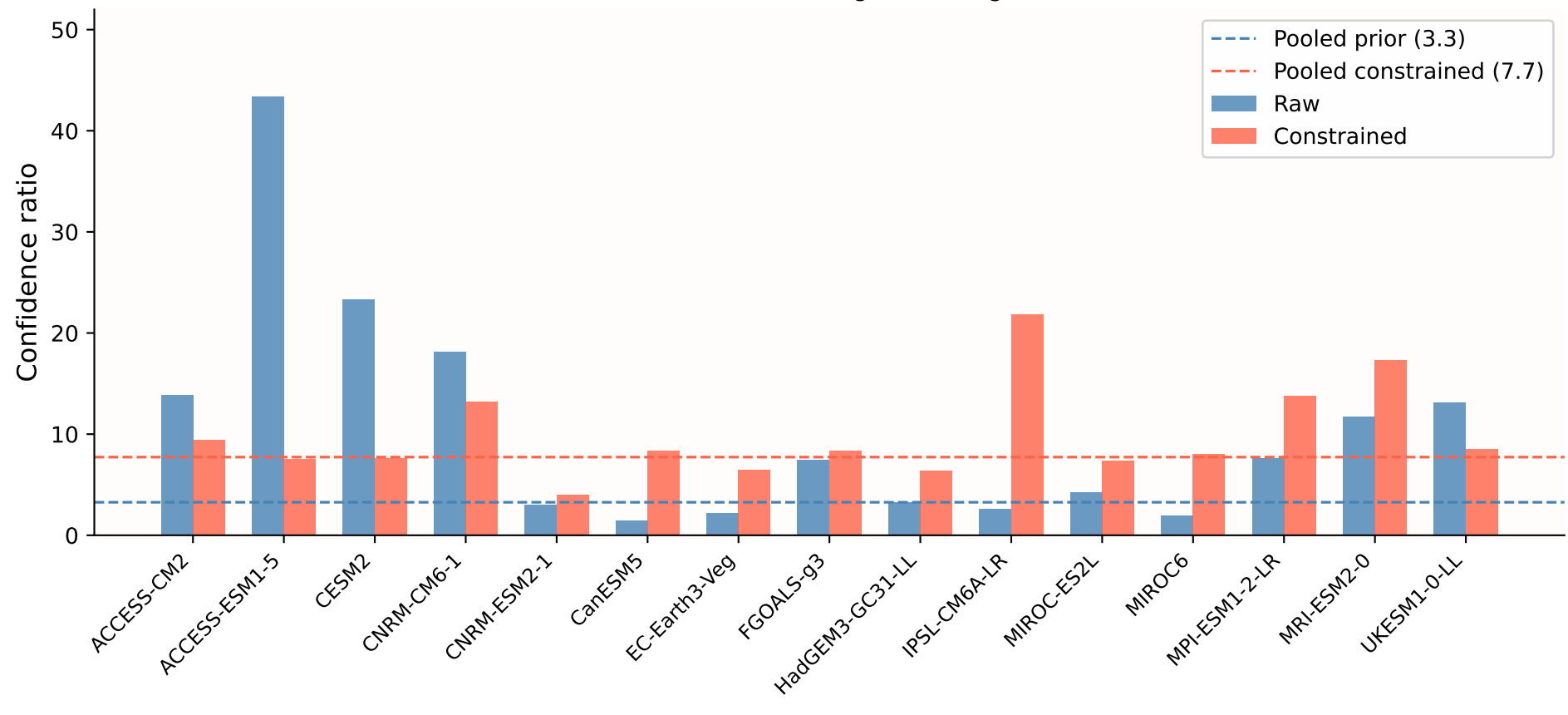
Global Land (LSAT): confidence ratio per pseudo-observation model Raw vs. Constrained (global + regional)
