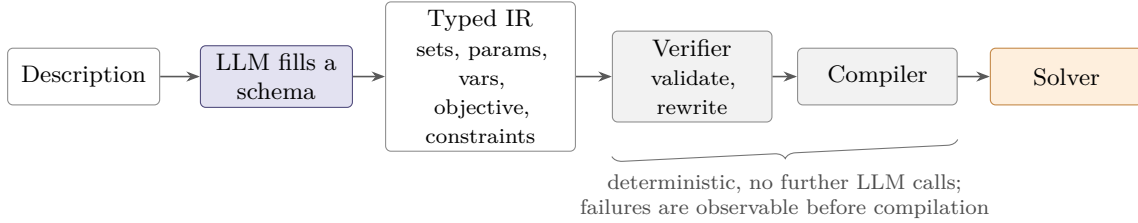
Figure 6: Direct code generation versus a structured intermediate representation (IR). In (b) the LLM fills a schema-constrained representation, and deterministic tools validate, rewrite, and compile it, as in IR2Solve [227]. R2C’s canonical representation and ORPilot’s solver-agnostic IR follow the same division of labor [110, 183]. Colors: blue, LLM steps; gray, deterministic tools or stored state; green, the user; orange, the solver. Dashed arrows are feedback.
