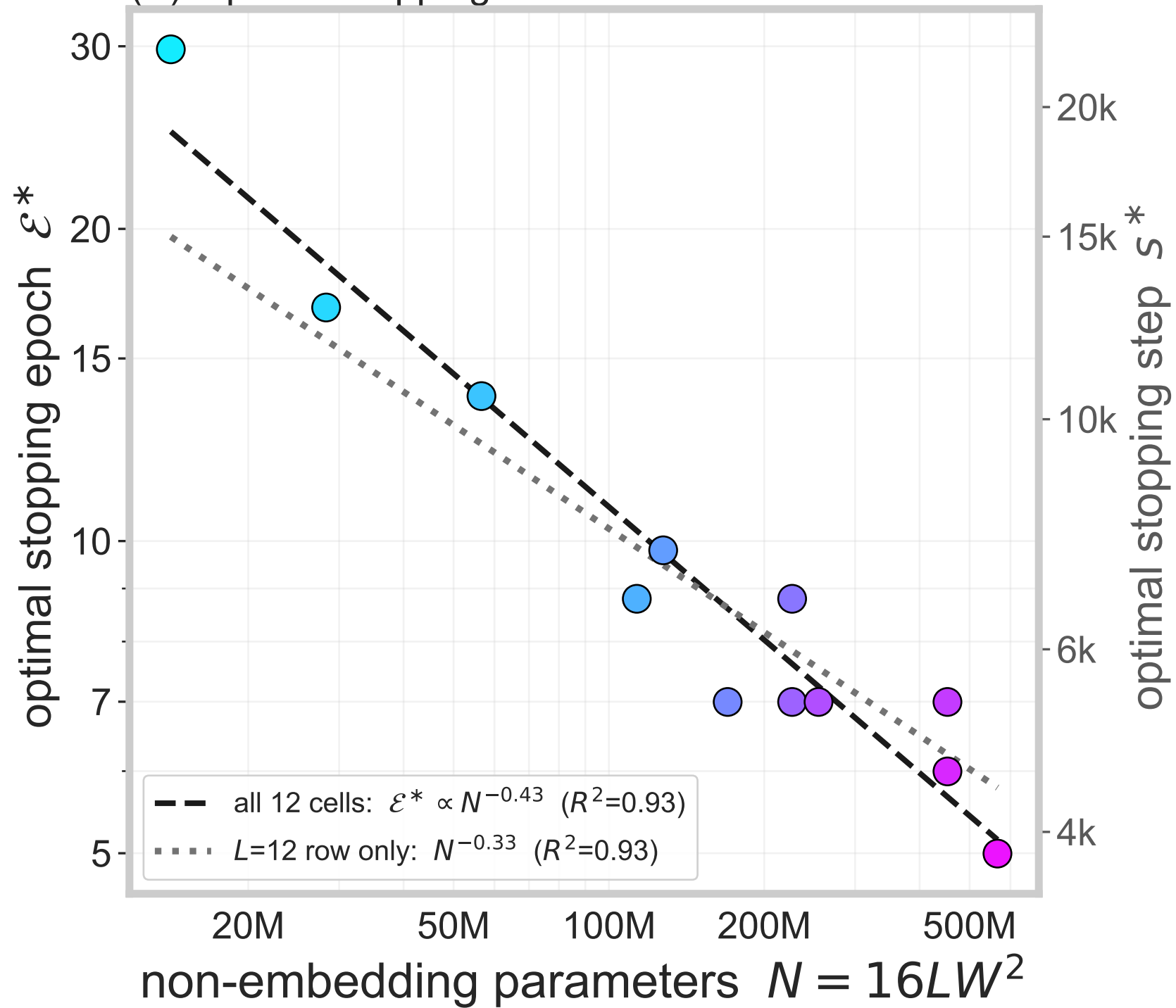
(A) optimal stopping shortens with model size
