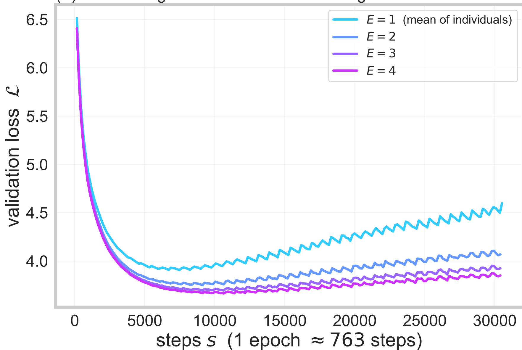
(A) ensembling reduces loss across training
