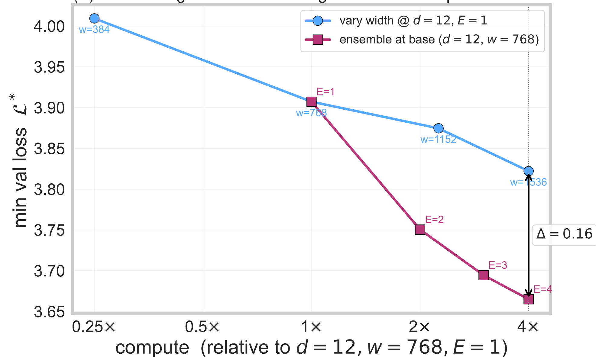
(B) ensembling beats width-scaling at matched compute
