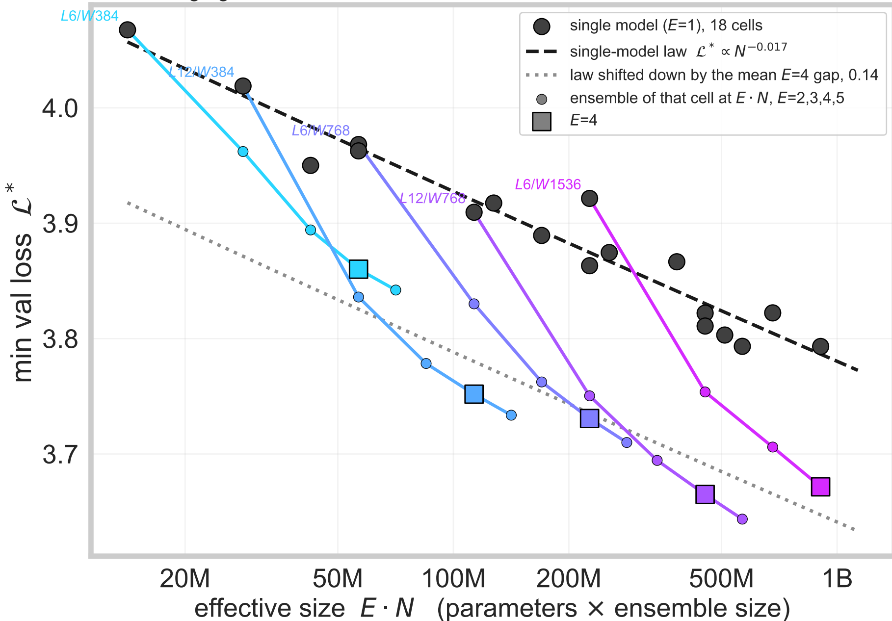
Ensembling against model size: each branch is one cell's ensemble series
