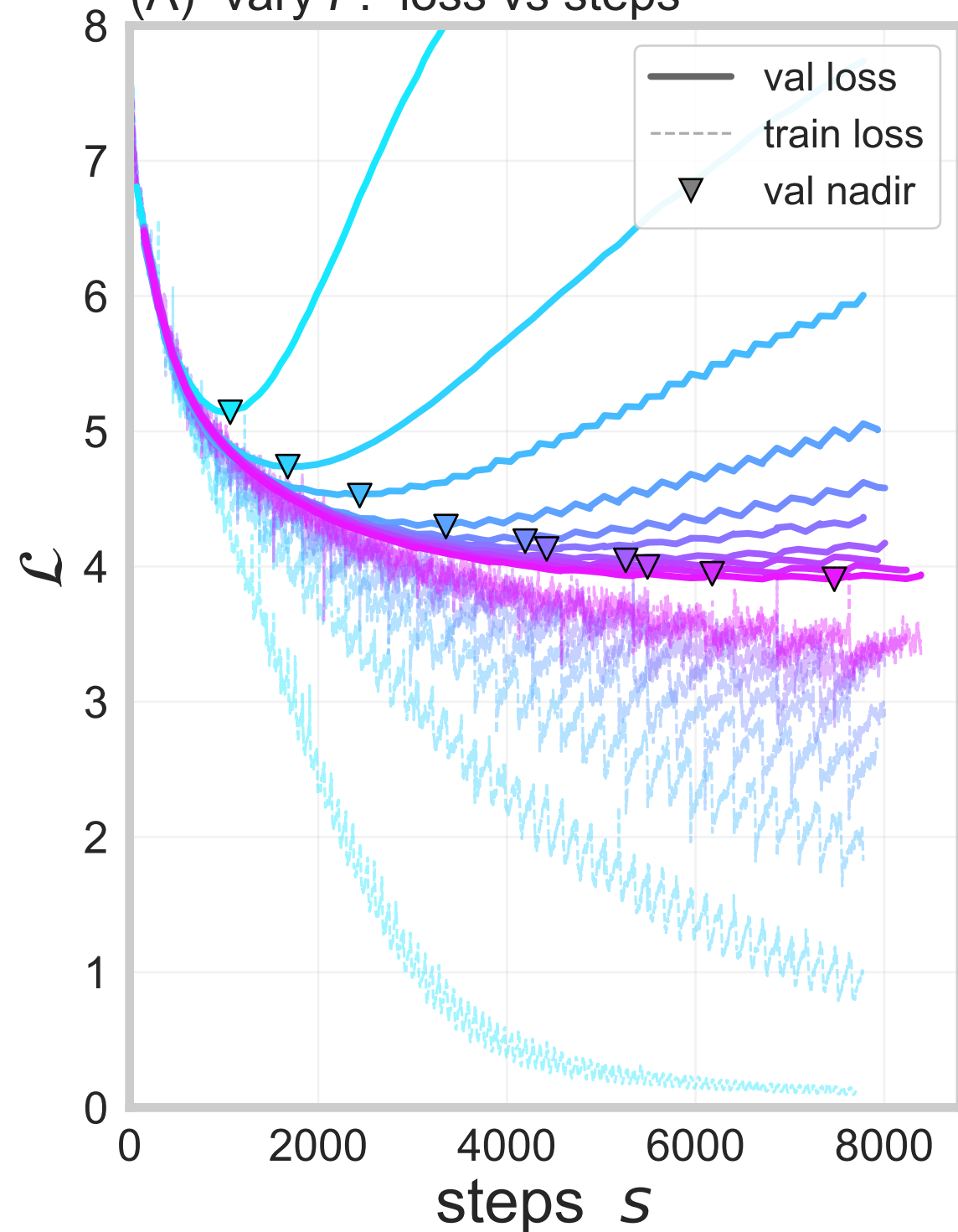
(A) vary P : loss vs steps
