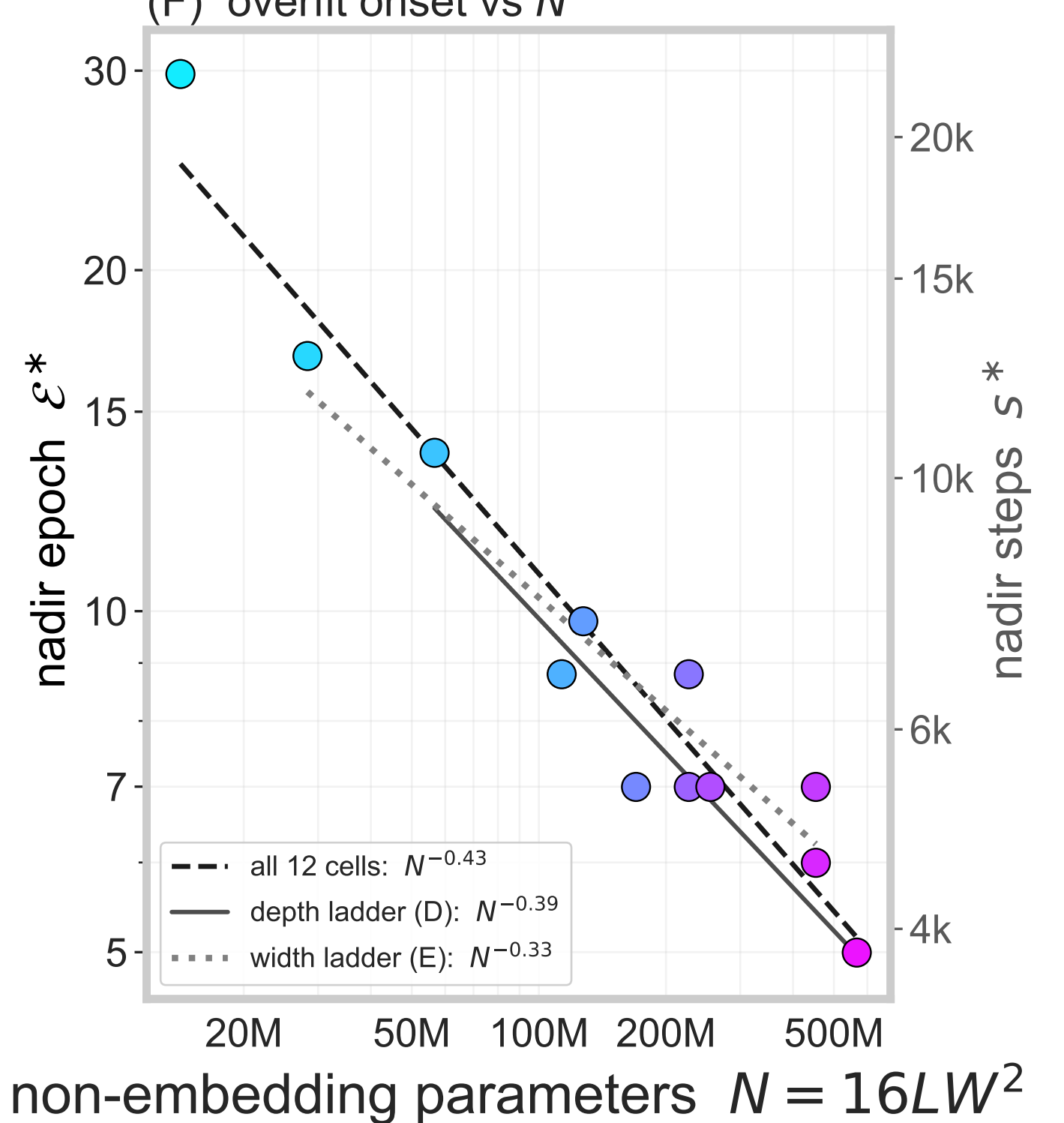
(F) overfit onset vs N
