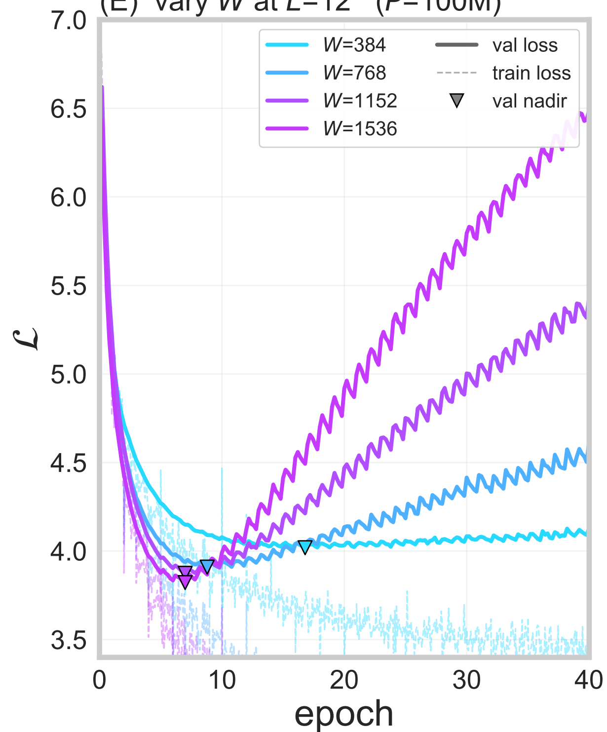
(E) vary W at L=12 ( P=100M )
