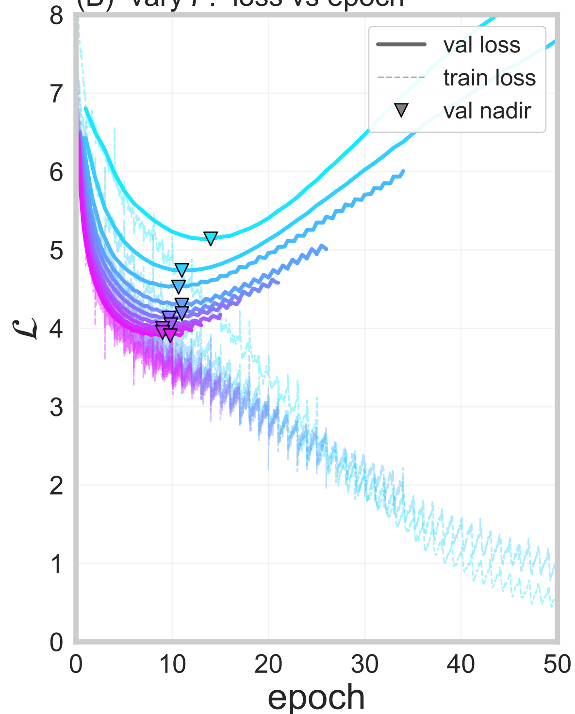
(B) vary P : loss vs epoch
