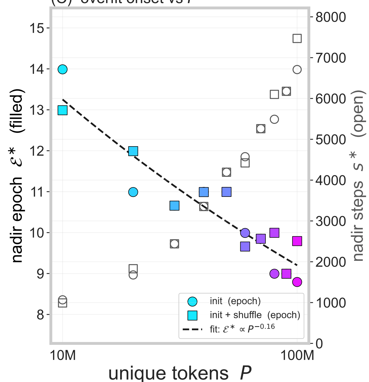
(C) overfit onset vs P
