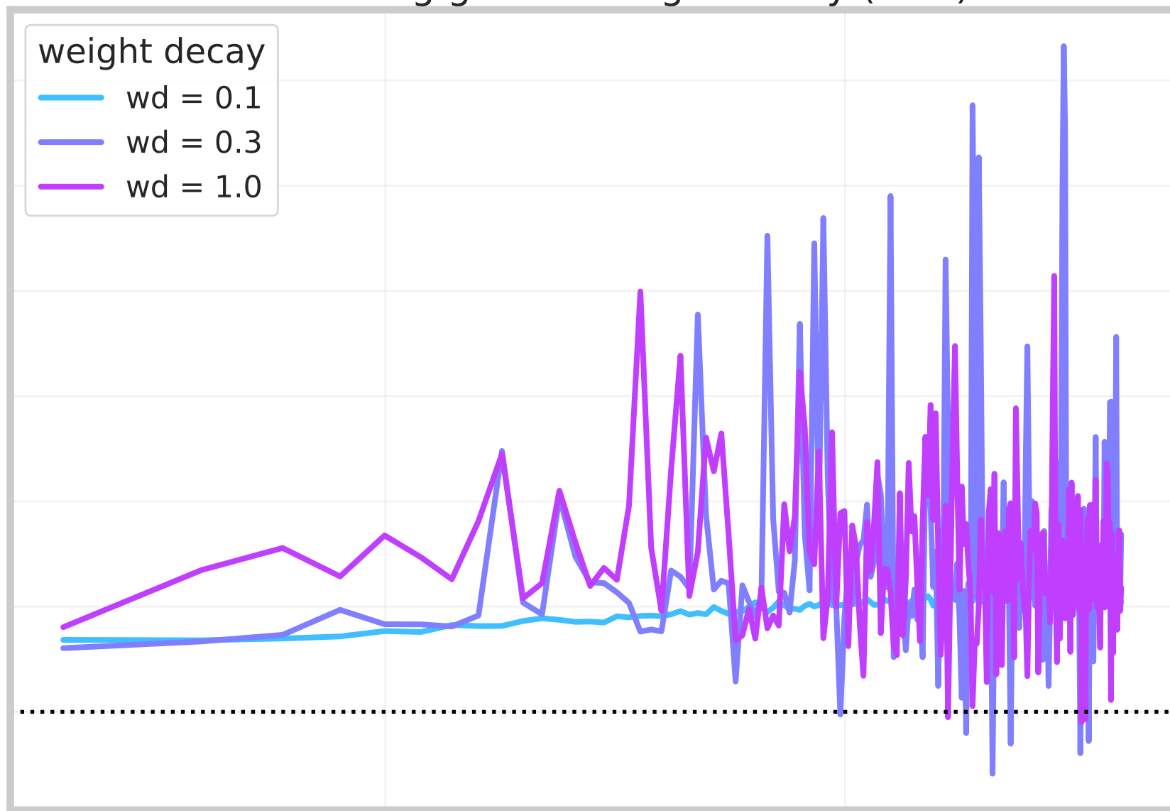
Ensembling gain vs weight decay (E=5)
