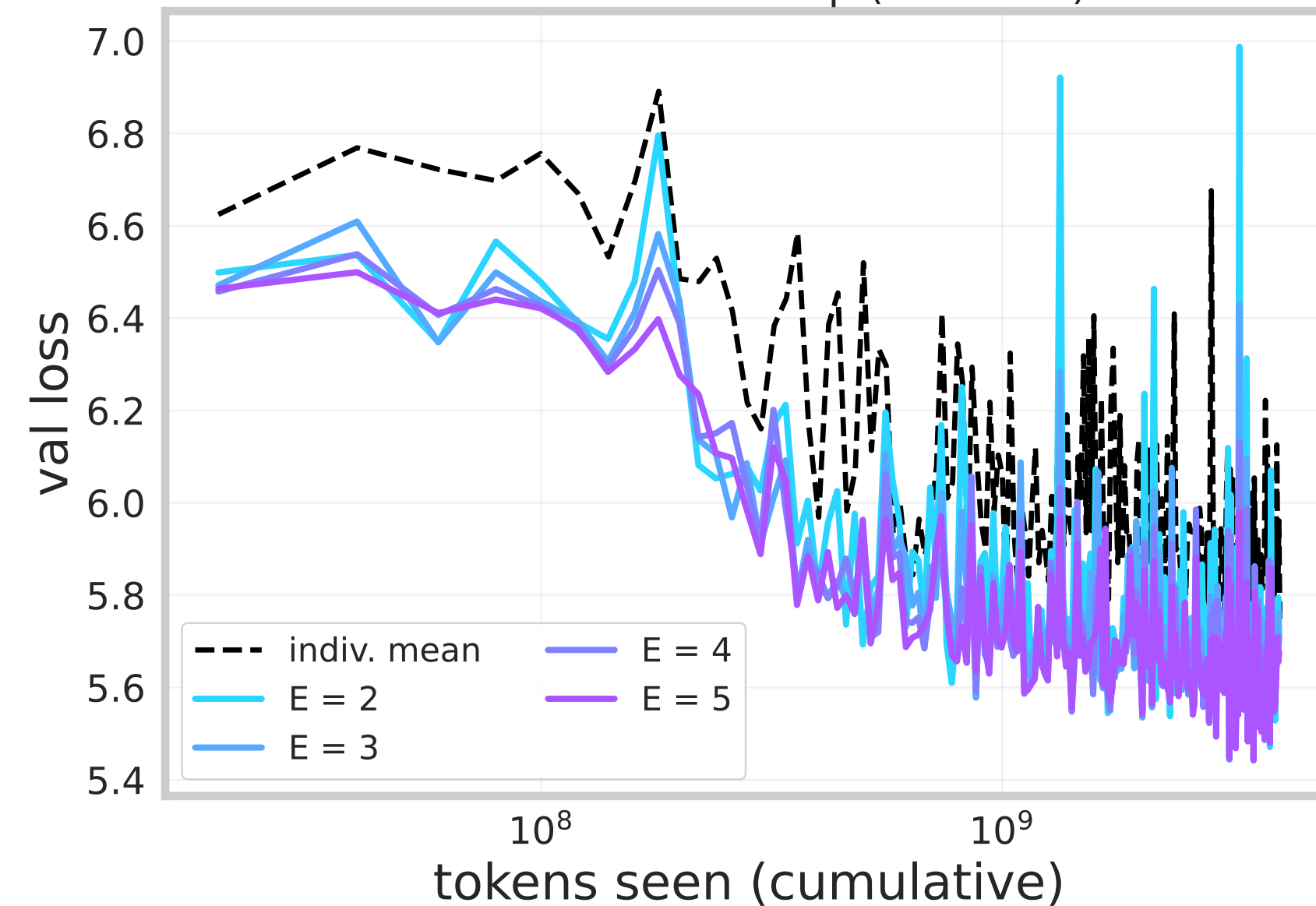
Ensemble size sweep (wd = 1.0)
