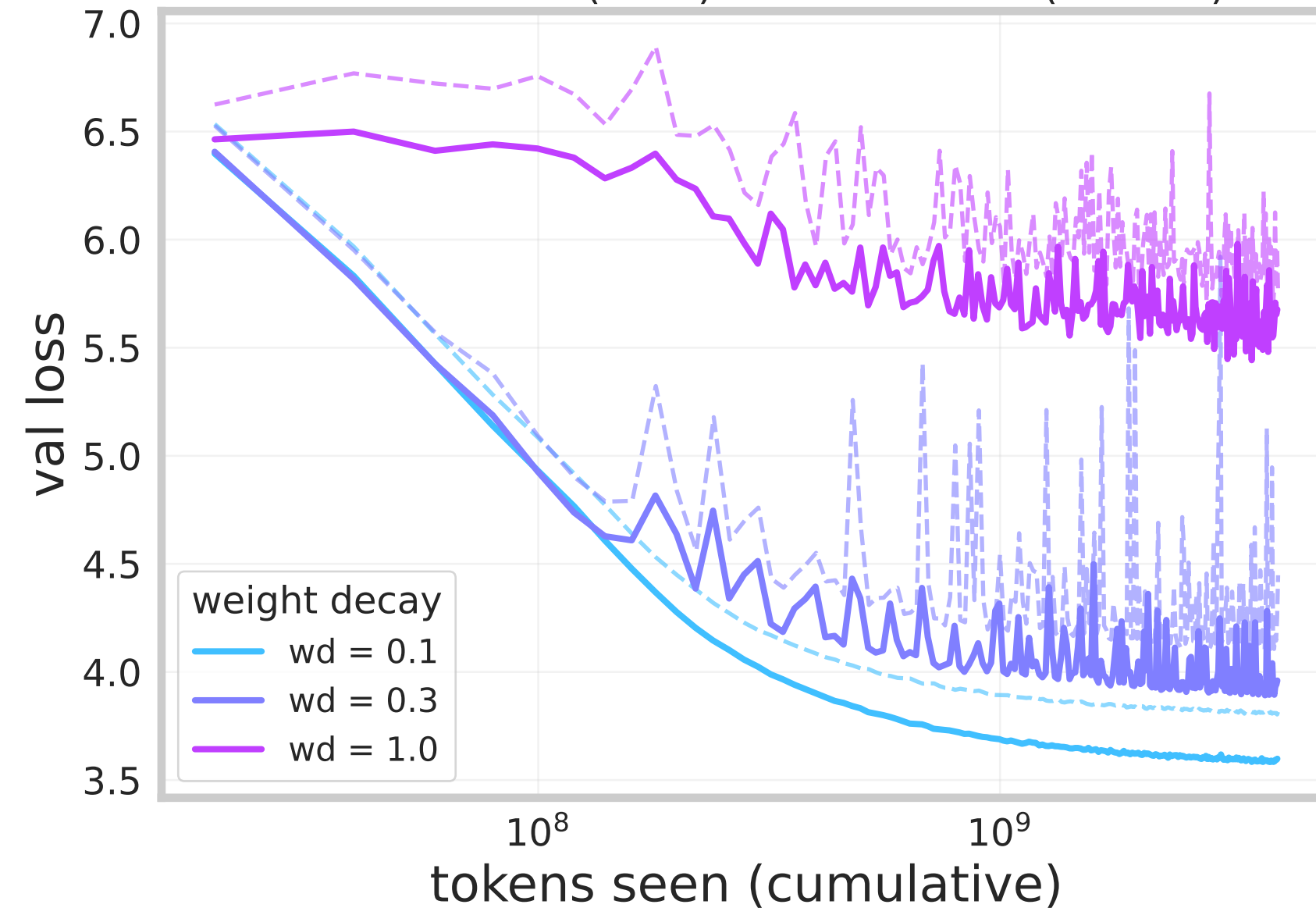
Ensemble E=5 (solid) vs indiv. mean (dashed)
