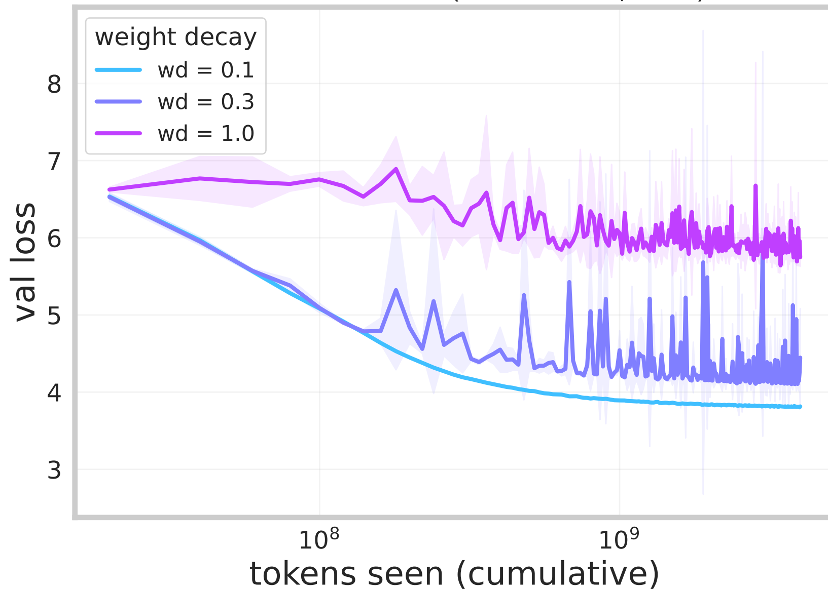
Individual models (mean ± std, N=5)
