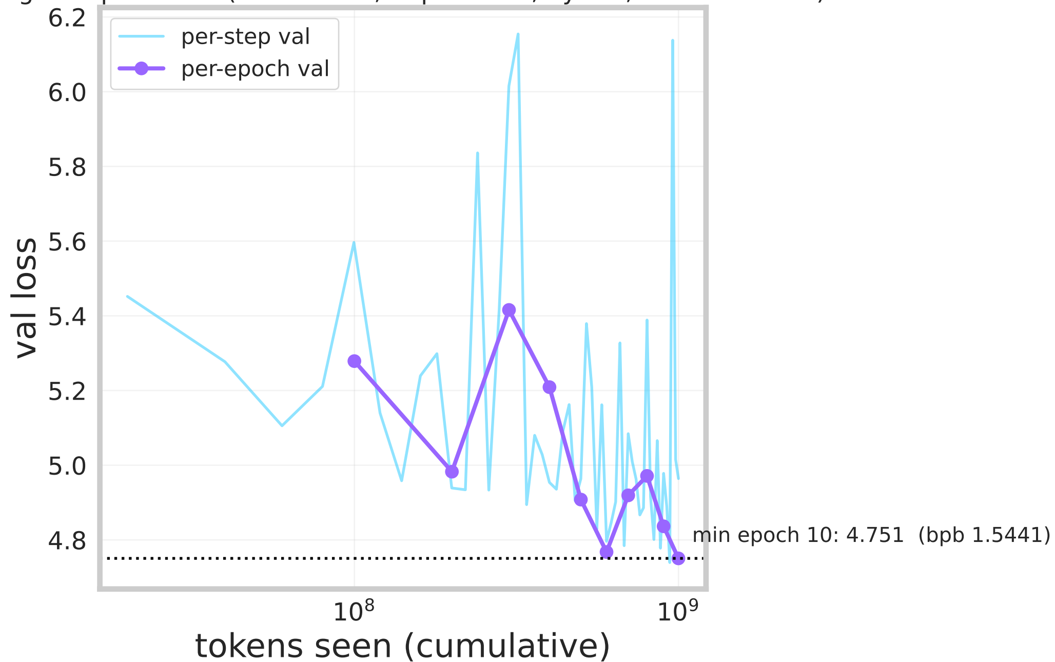
Single looped 1.8B (d30 w2048, dupe 15-25, hybrid, no-warmdown)
