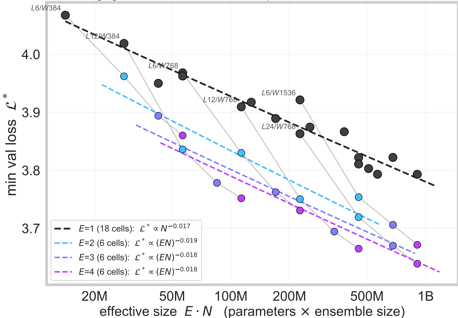
Ensembling against model size: one fitted law per ensemble size
