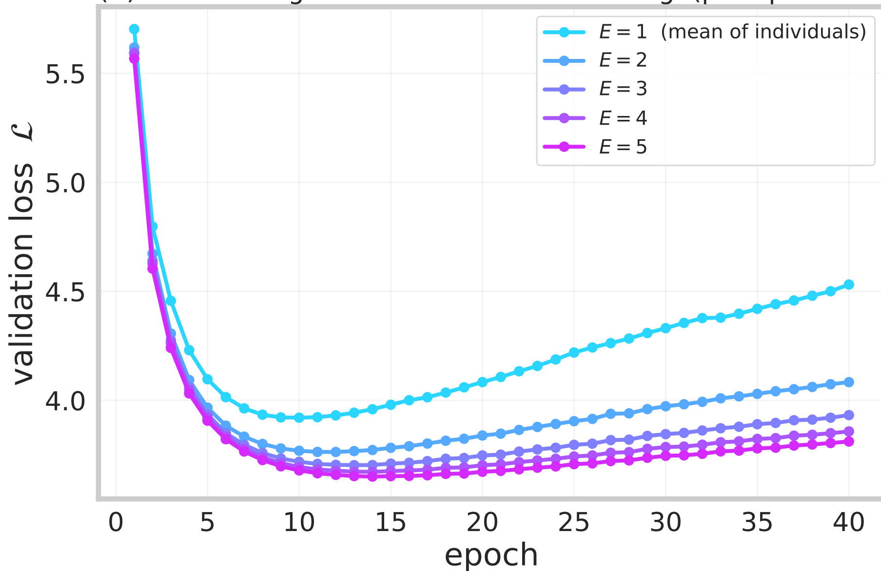
(A) ensembling reduces loss across training (per-epoch mean)
