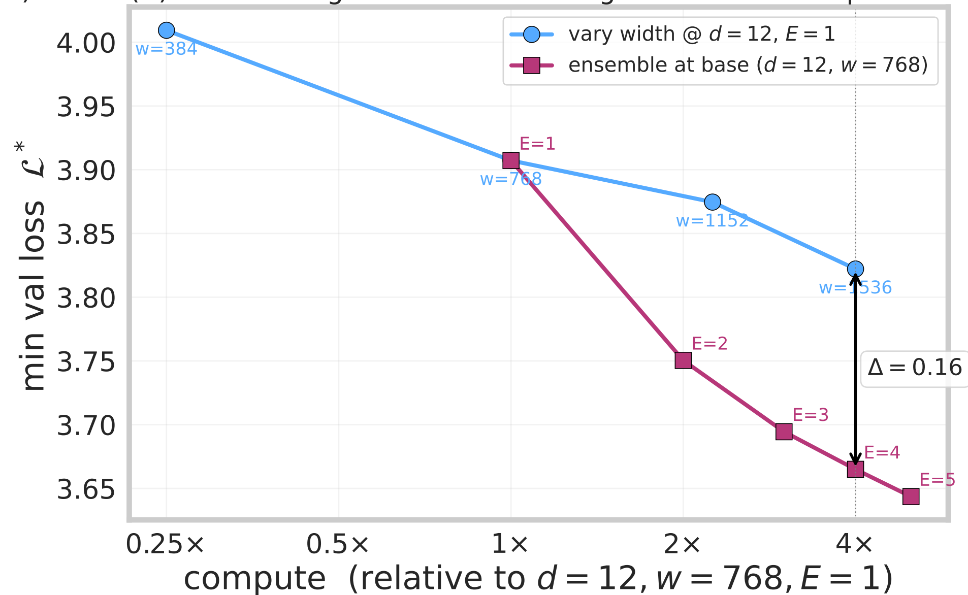
(B) ensembling beats width-scaling at matched compute
