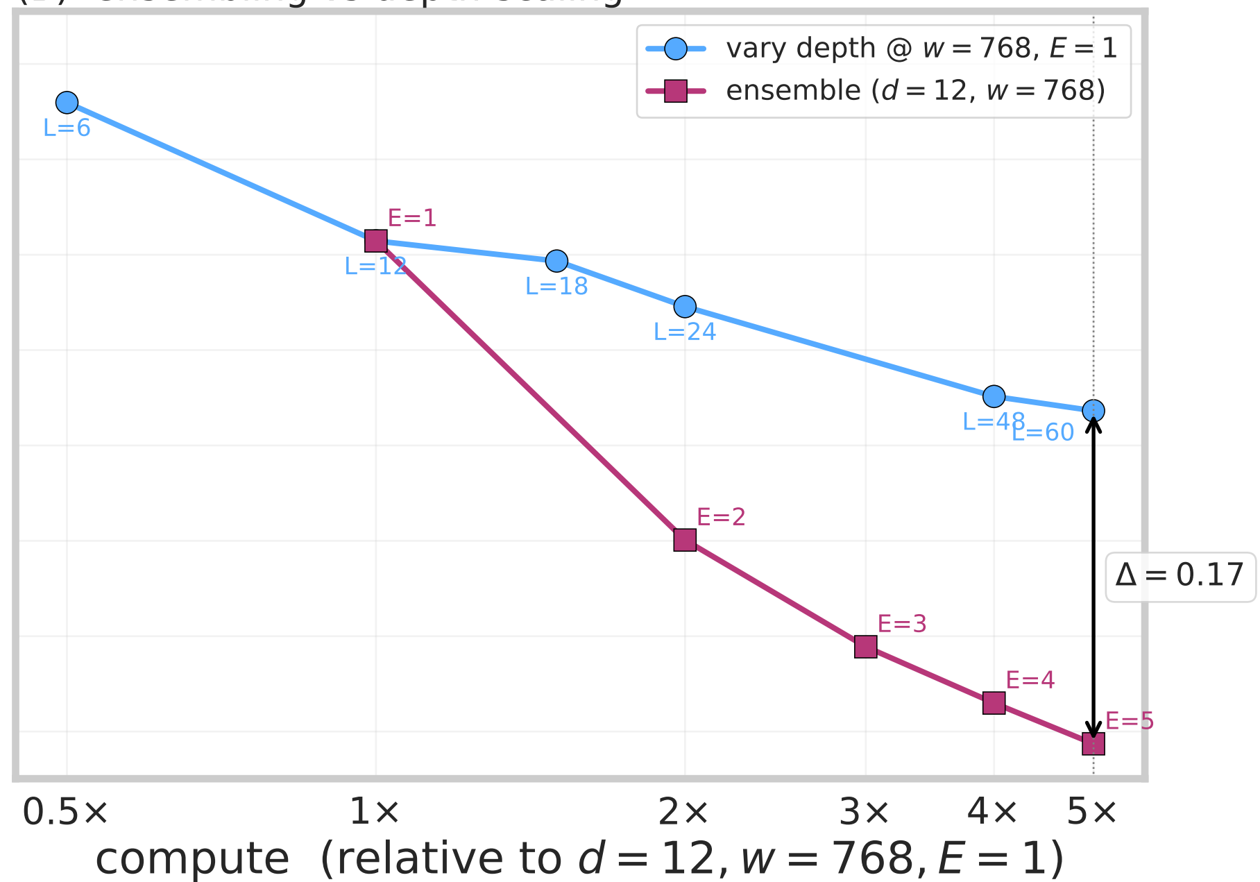
(B) ensembling vs depth-scaling
