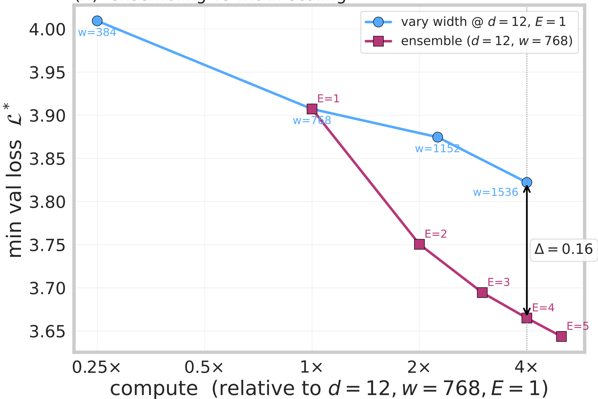
(A) ensembling vs width-scaling
