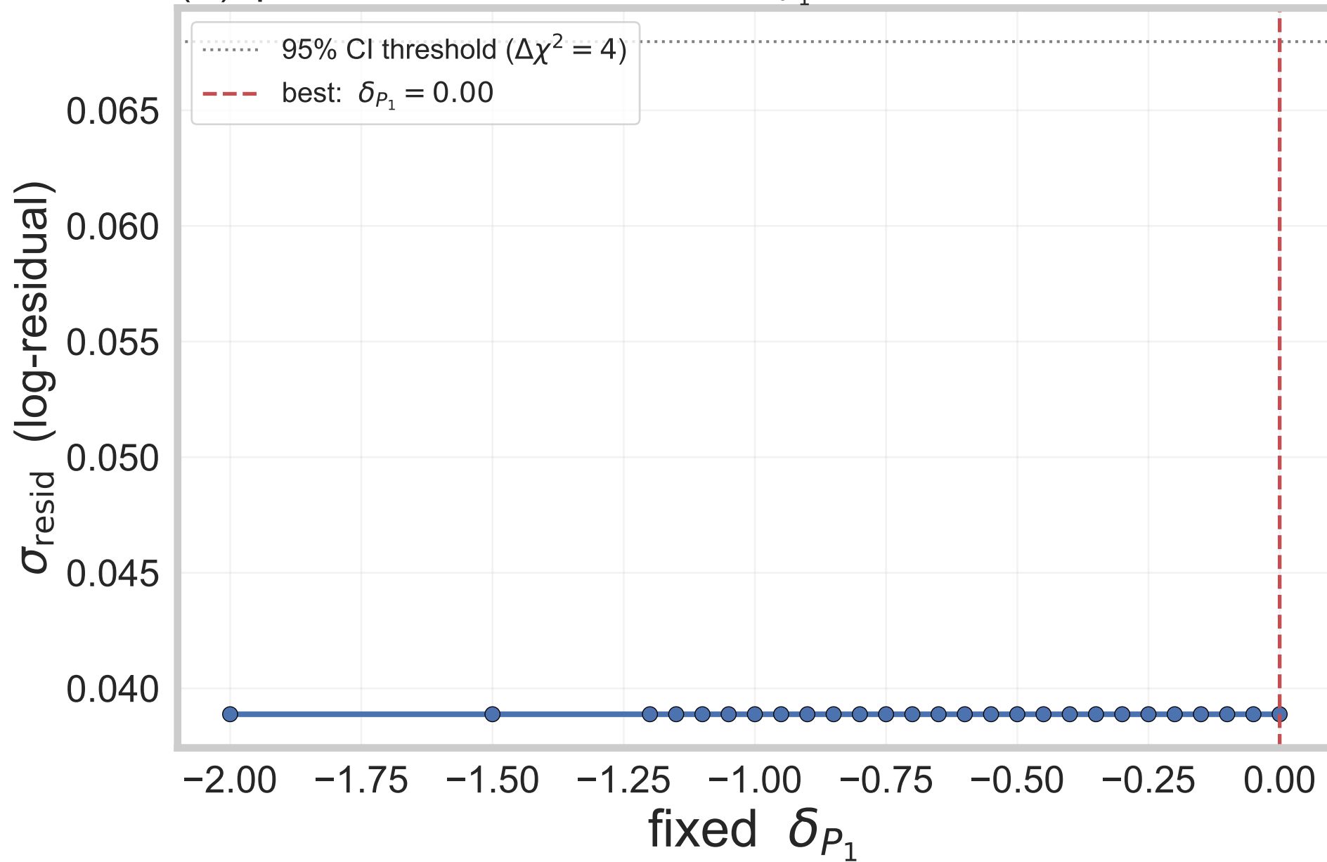
(A) profile-likelihood scan over \delta_{P_1}
