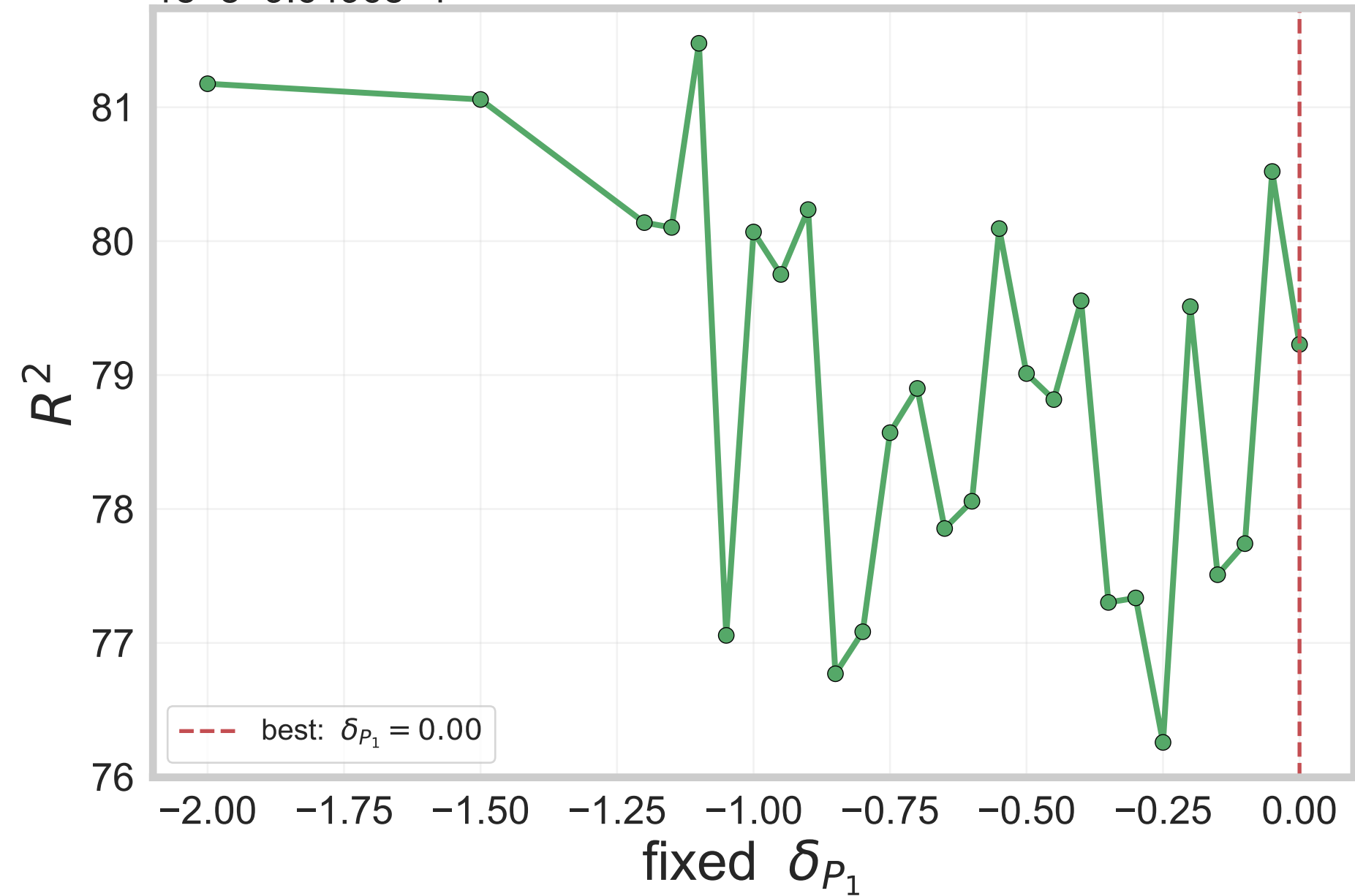
(B) R^2 vs \delta_{P_1} 1e-8+9.6496e-1
