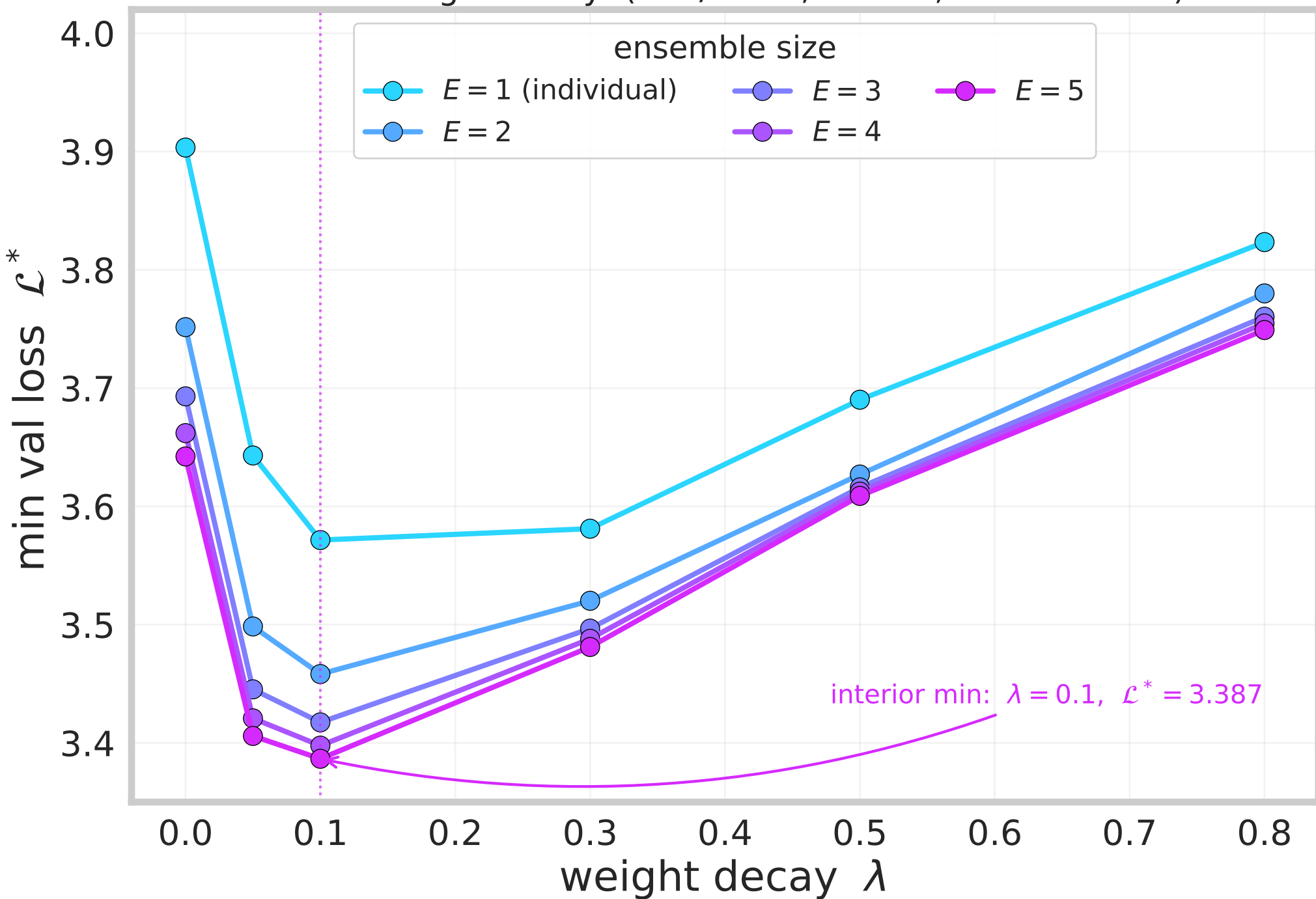
Min val loss vs weight decay (d12/w768, df=1.0, cooldown ON)
