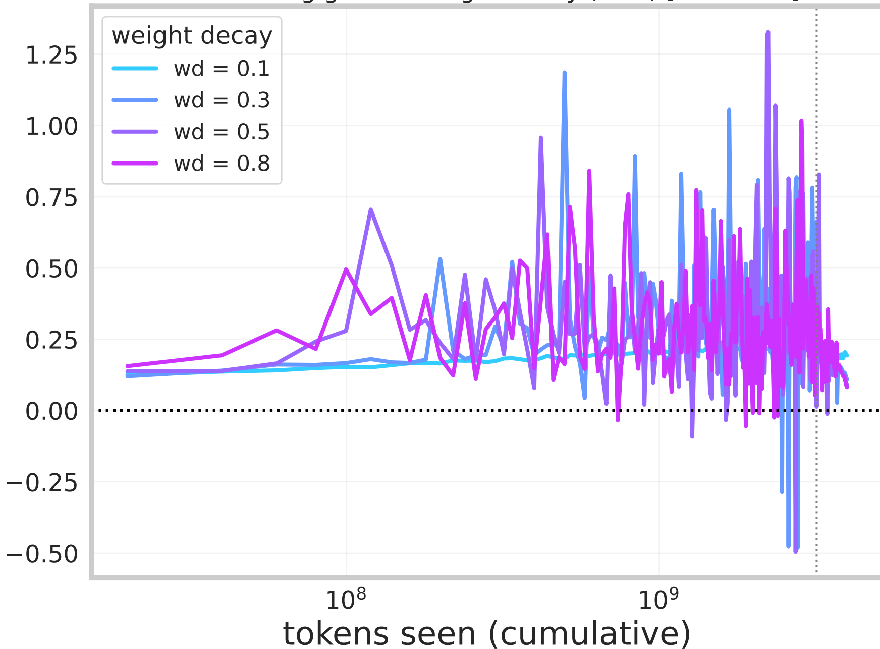
Ensembling gain vs weight decay (E=5) [cooldown]
