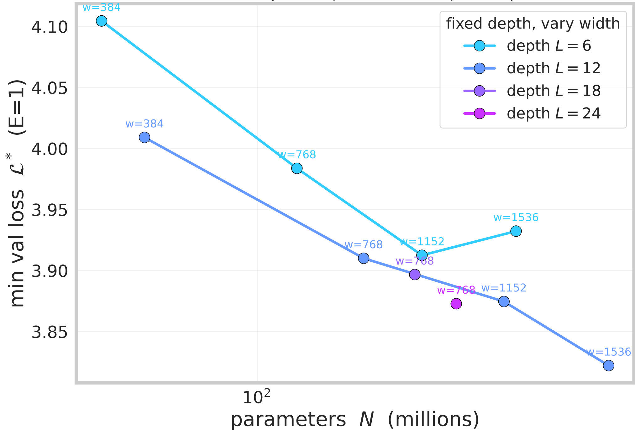
Val loss vs model size (df=1.0, 100M tokens, wd=0)
