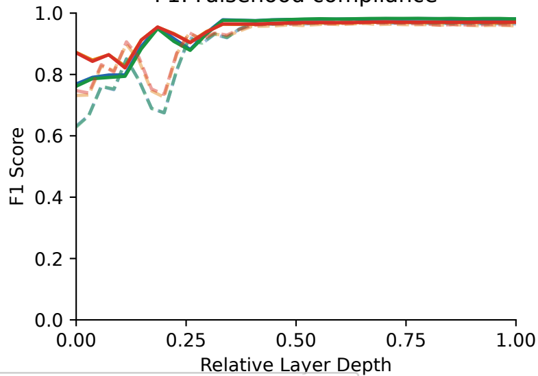
F1: Falsehood compliance
