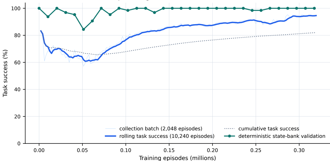
PPO whip learning and held-out initial-state validation
