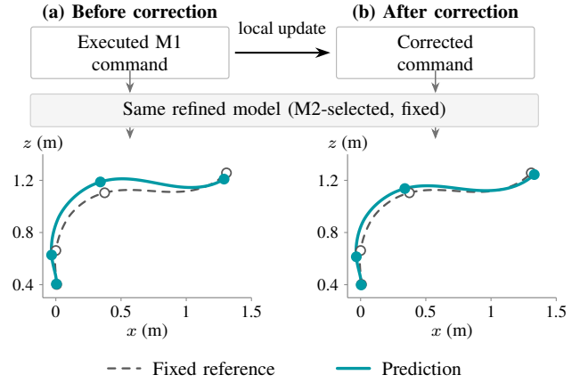
Fig. 2: Saved tip predictions before and after command correction with the fixed M2-selected model, shown in the world x - z plane. Both panels use the original MPPI reference; markers pair equal timestamps. Curves are simulation predictions, not measurements.
