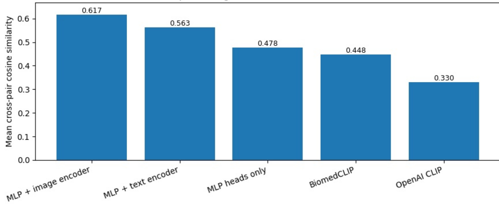
Cross-paired alignment score on held-out test set
