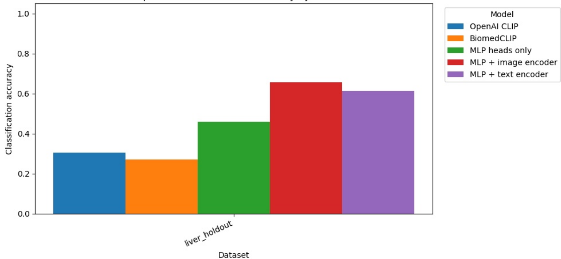
Prompt-based classification accuracy by dataset
