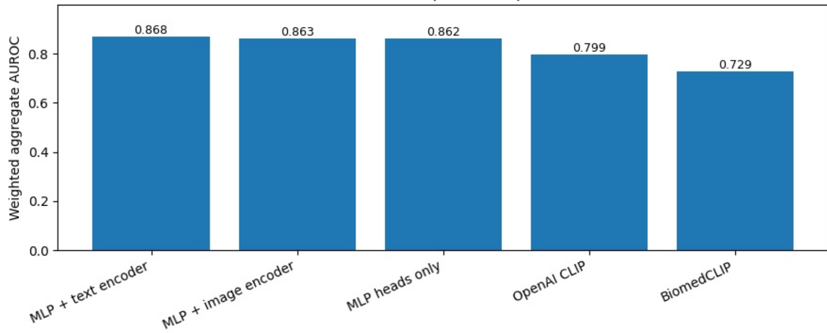
Held-out linear probe comparison
