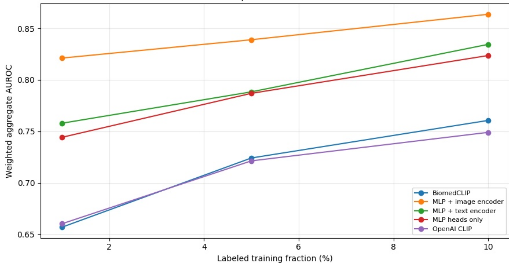
Few-shot adaptation on held-out test set
