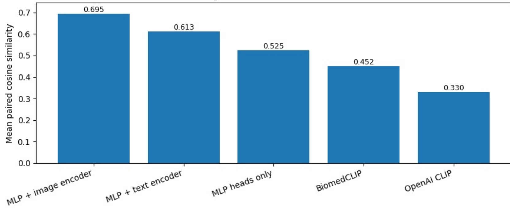
Paired alignment score on held-out test set
