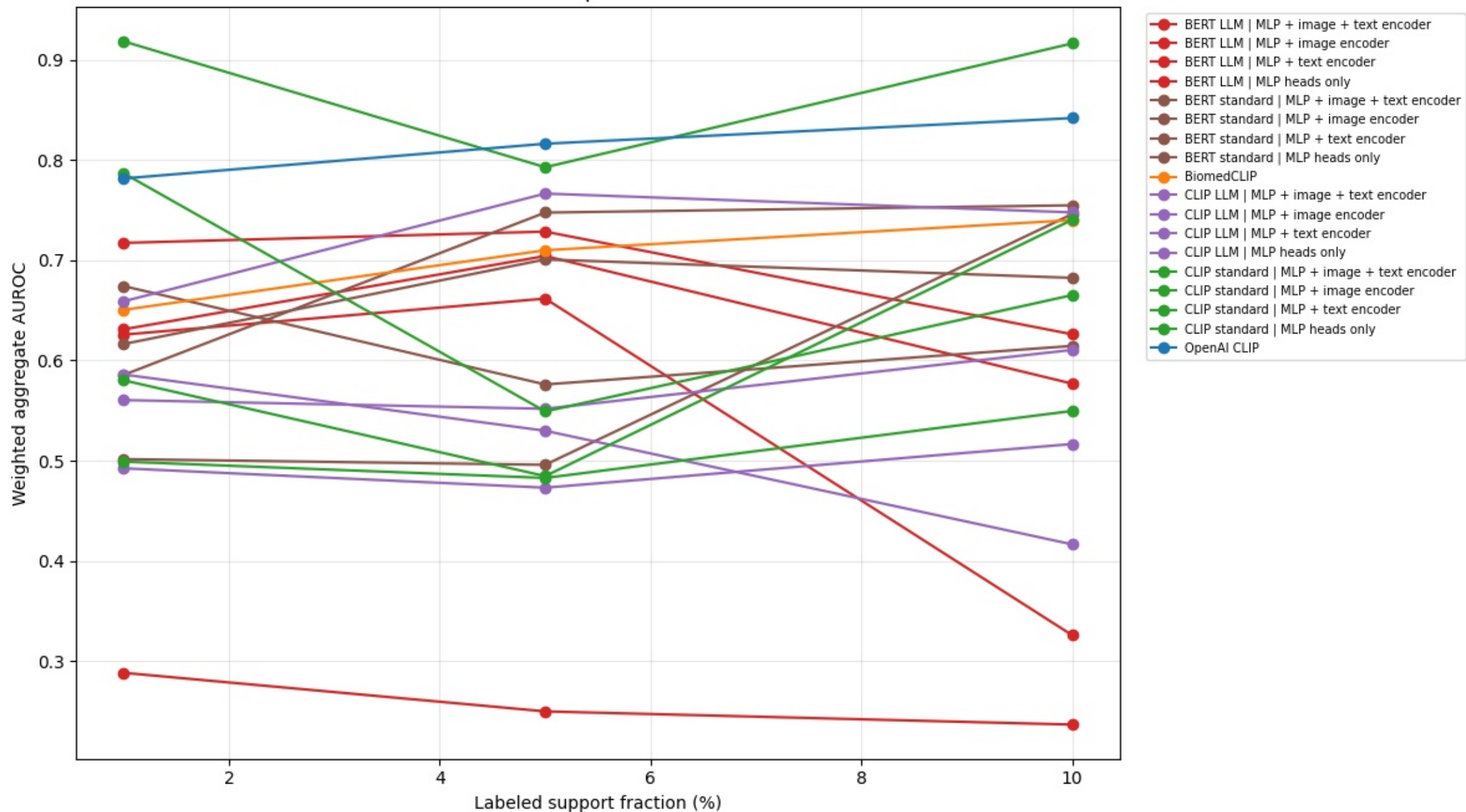
End-to-end few-shot adaptation on liver holdout set
