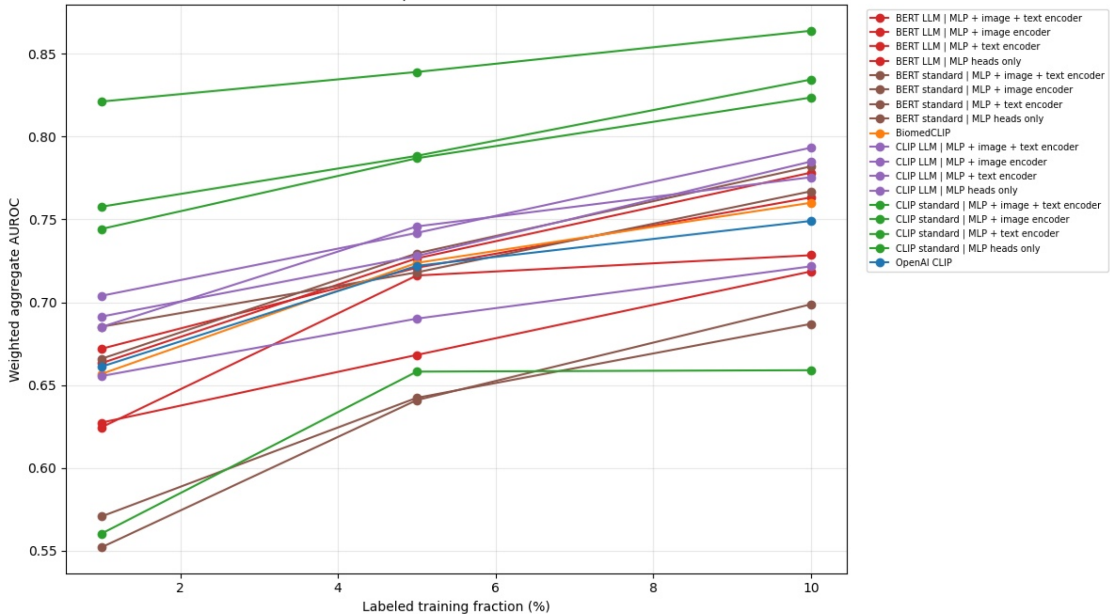
Few-shot adaptation on liver holdout set
