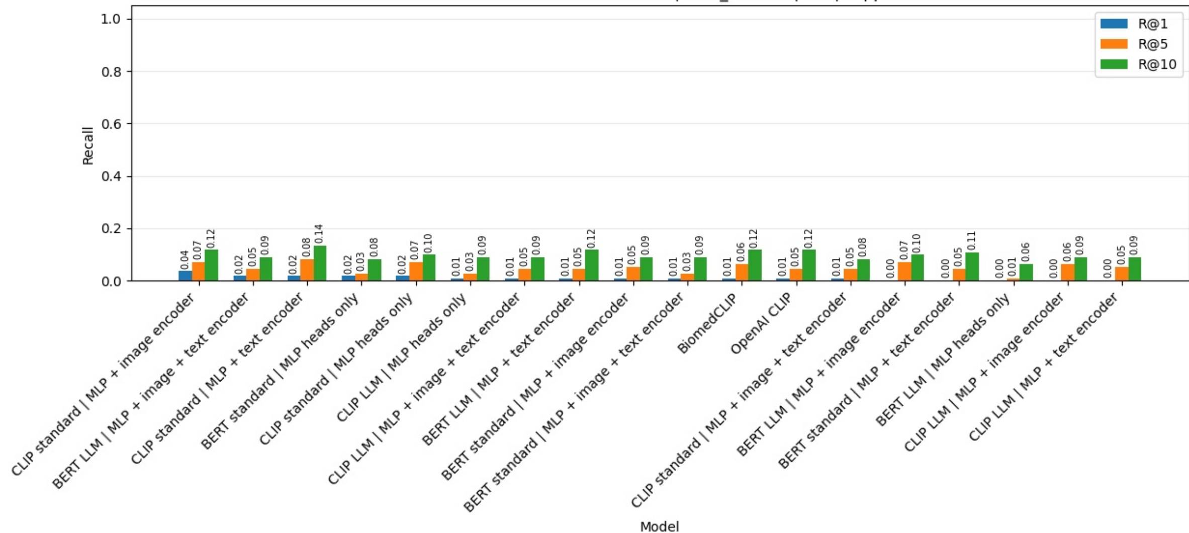
Few-shot retrieval on liver holdout set | liver_holdout | T2I | support=10%
