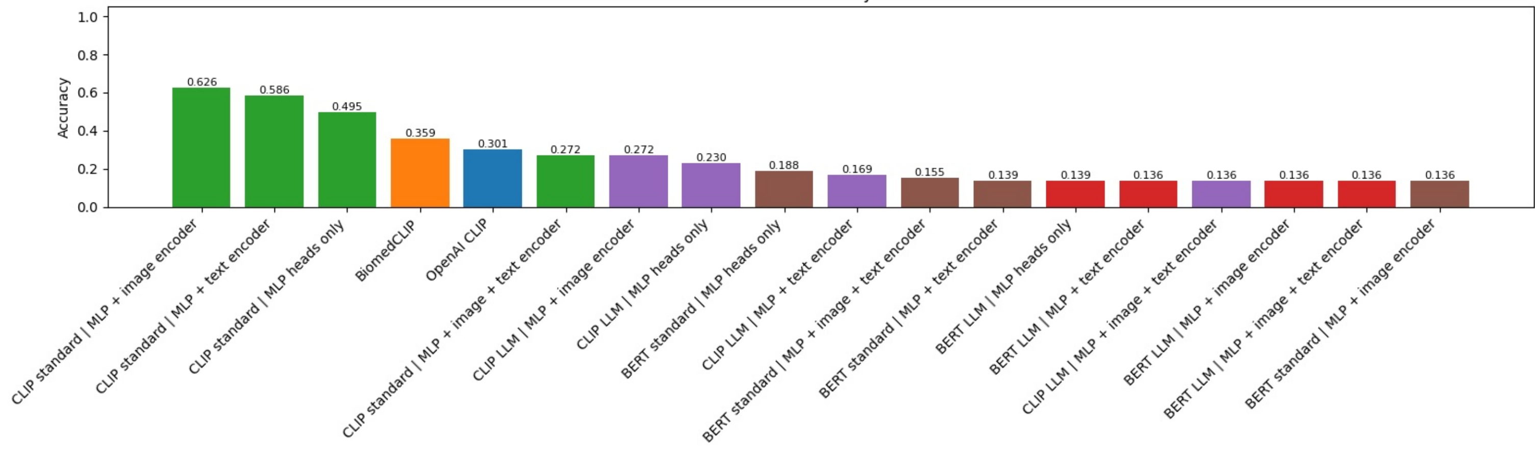
Zero-shot classification accuracy on liver holdout set
