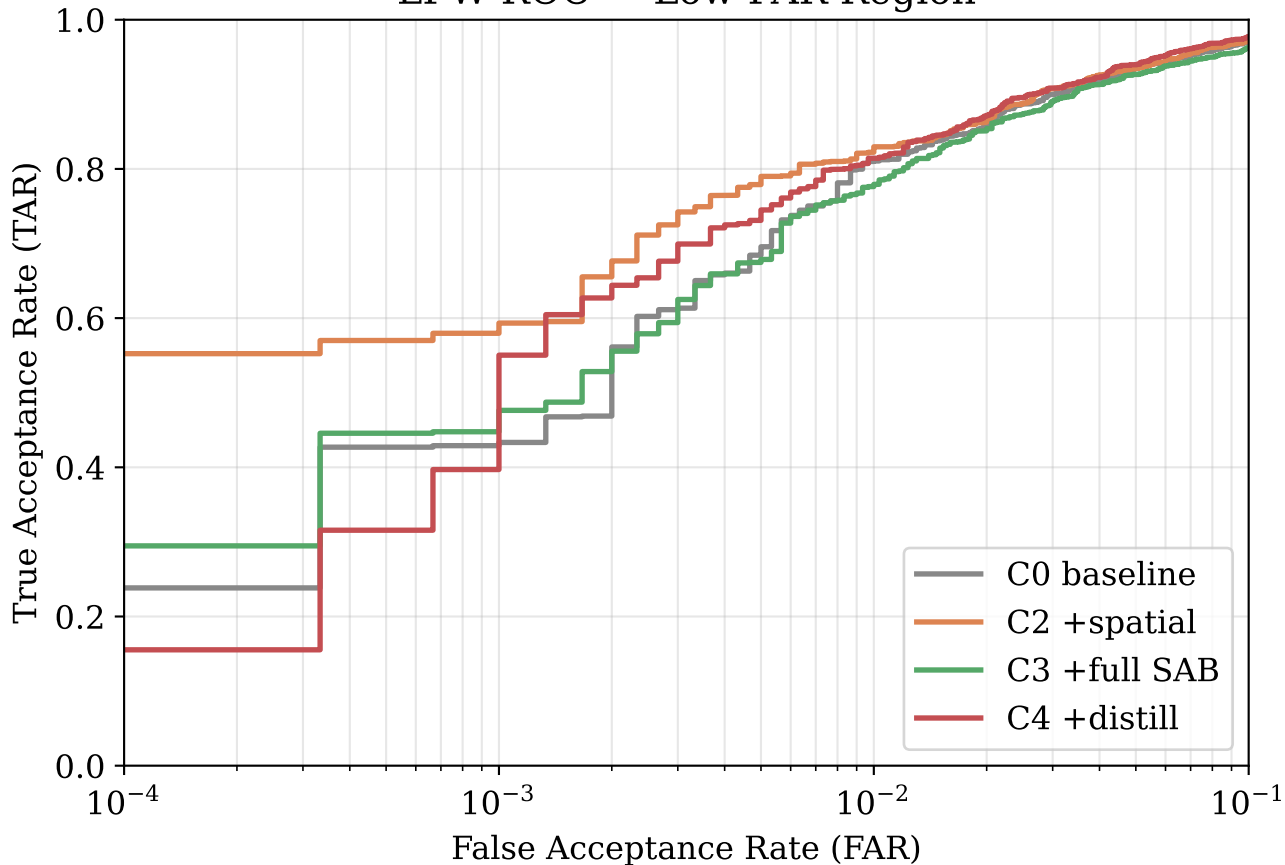
LFW ROC — Low-FAR Region
