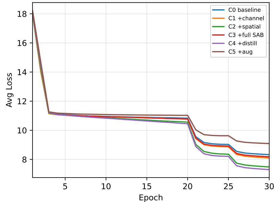
Training Loss
