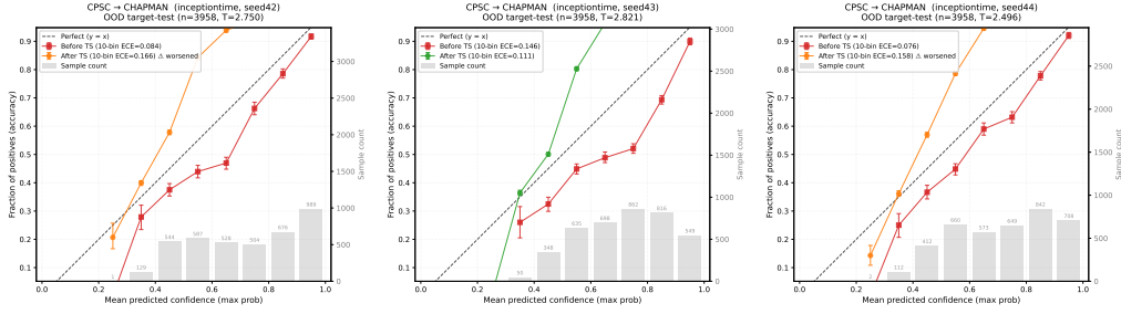
Figure 20: CPSC→Chapman reliability diagrams: InceptionTime seeds 42–44.
