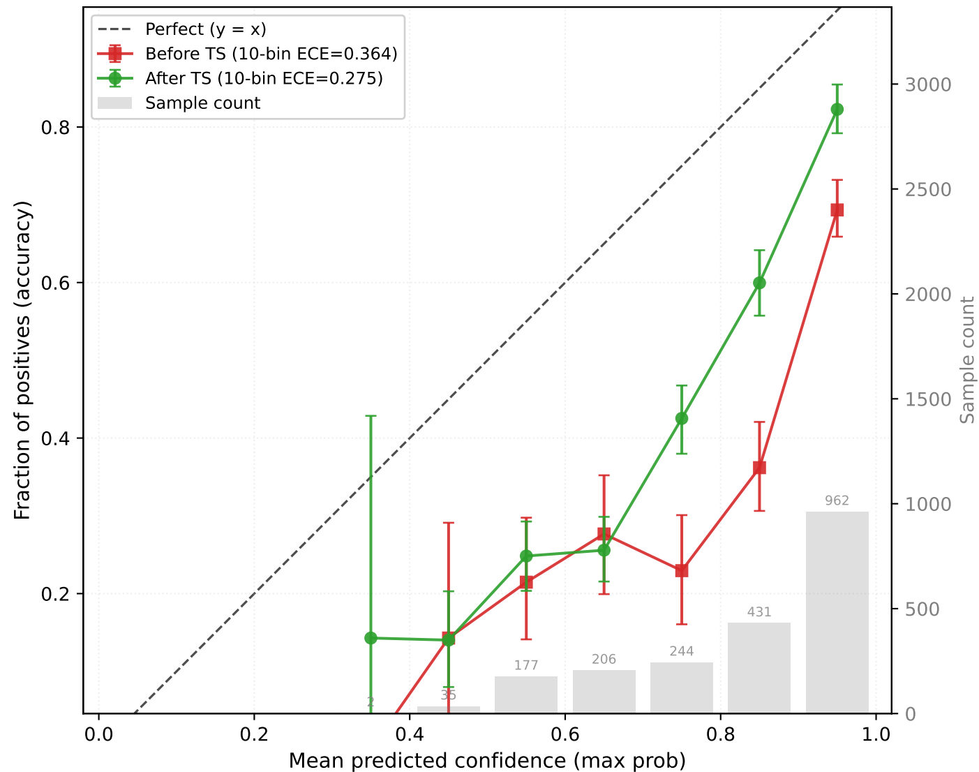
CHAPMAN → CPSC OOD target-test (n=2057, resnet1d, seed42, T=1.536)
