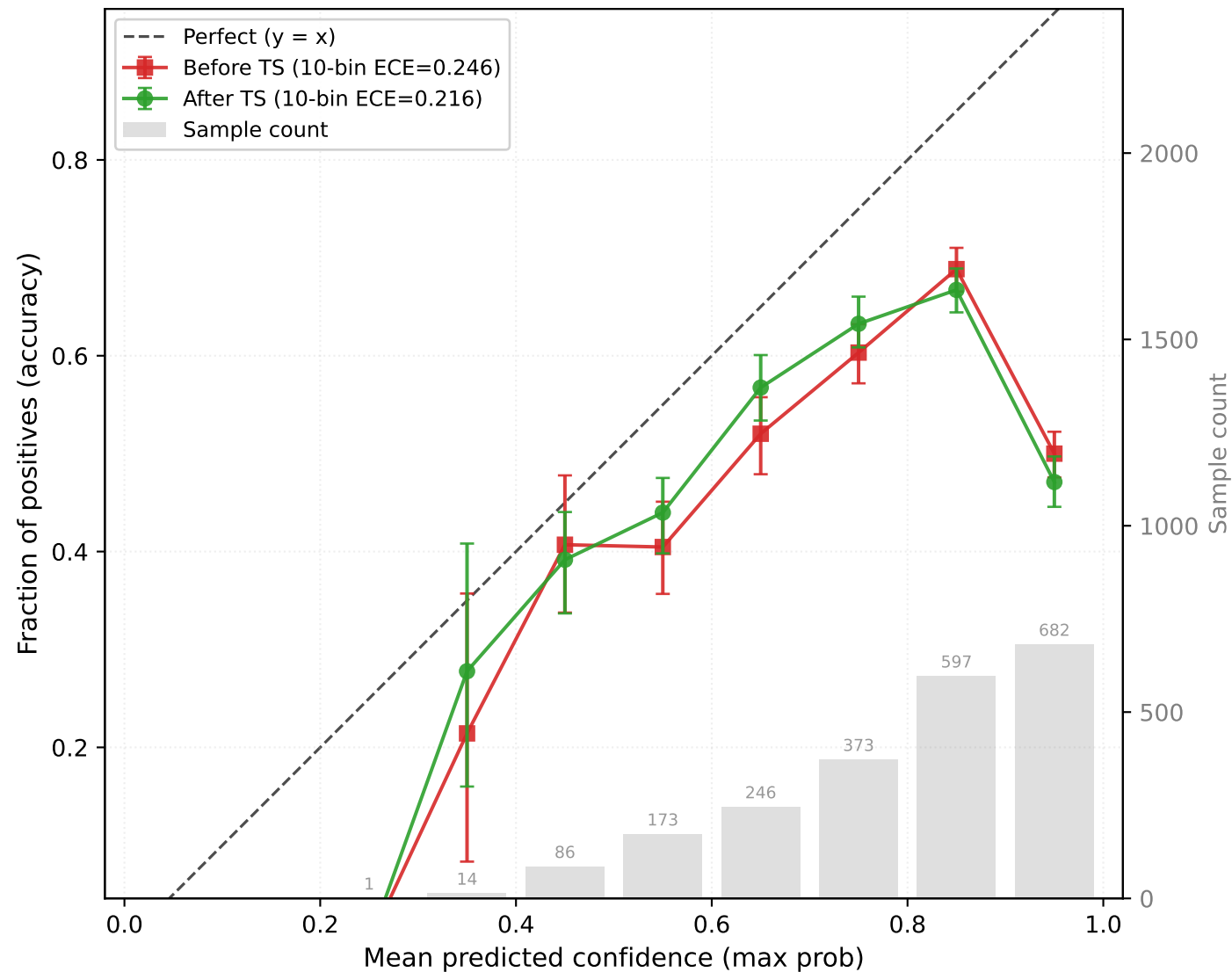
CHAPMAN → PTBXL OOD target-test (n=2172, resnet1d, seed42, T=1.125)
