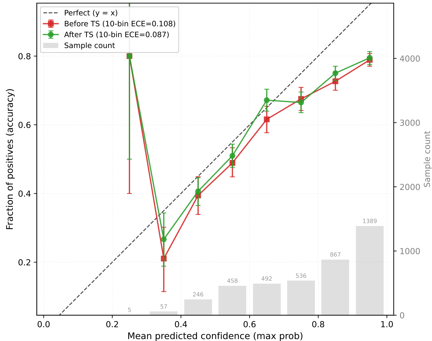
PTBXL → CHAPMAN OOD target-test (n=4050, resnet1d, seed42, T=1.108)
