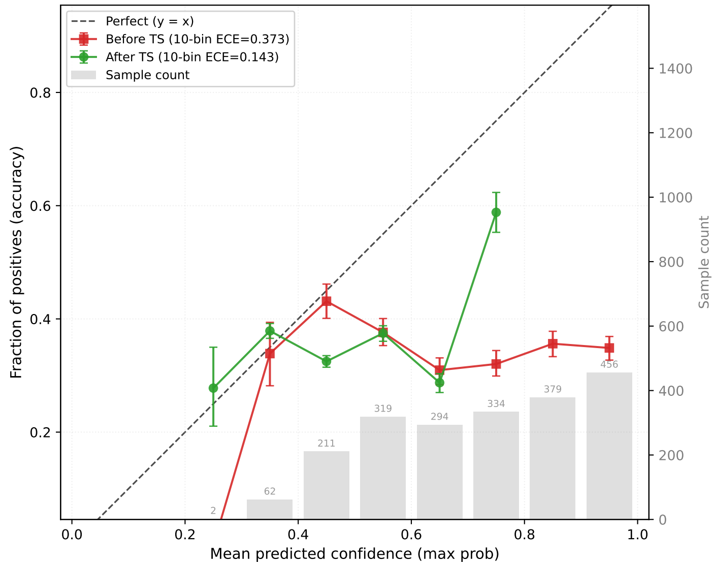
PTBXL \rightarrow CPSC OOD target-test (n=2057, resnet1d, seed42, T=2.529)
