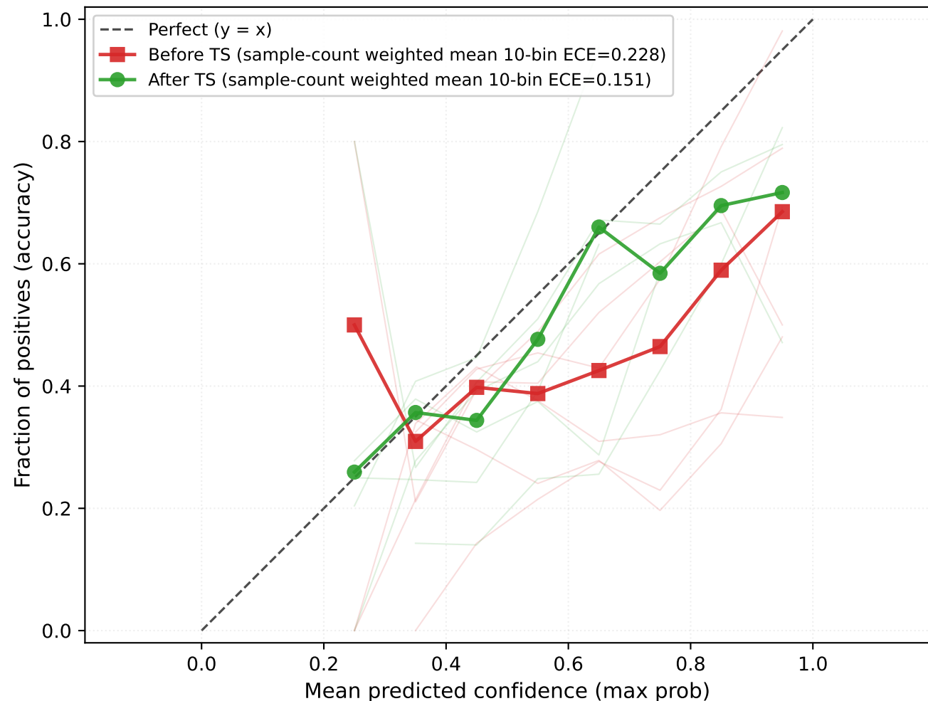
Summary: 6-direction averaged reliability curve (curve: bin-count weighted; ECE: sample-count weighted mean 10-bin; resnet1d, seed42) Background curves: inter-direction variability (not inter-seed)
