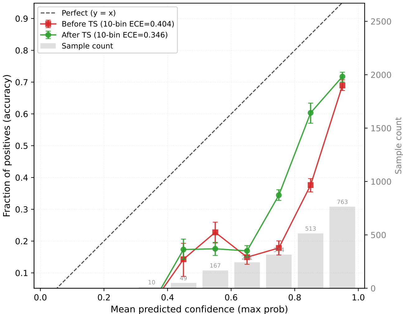
CHAPMAN → CPSC (resnet1d, seed46) OOD target-test (n=2057, T=1.344)
