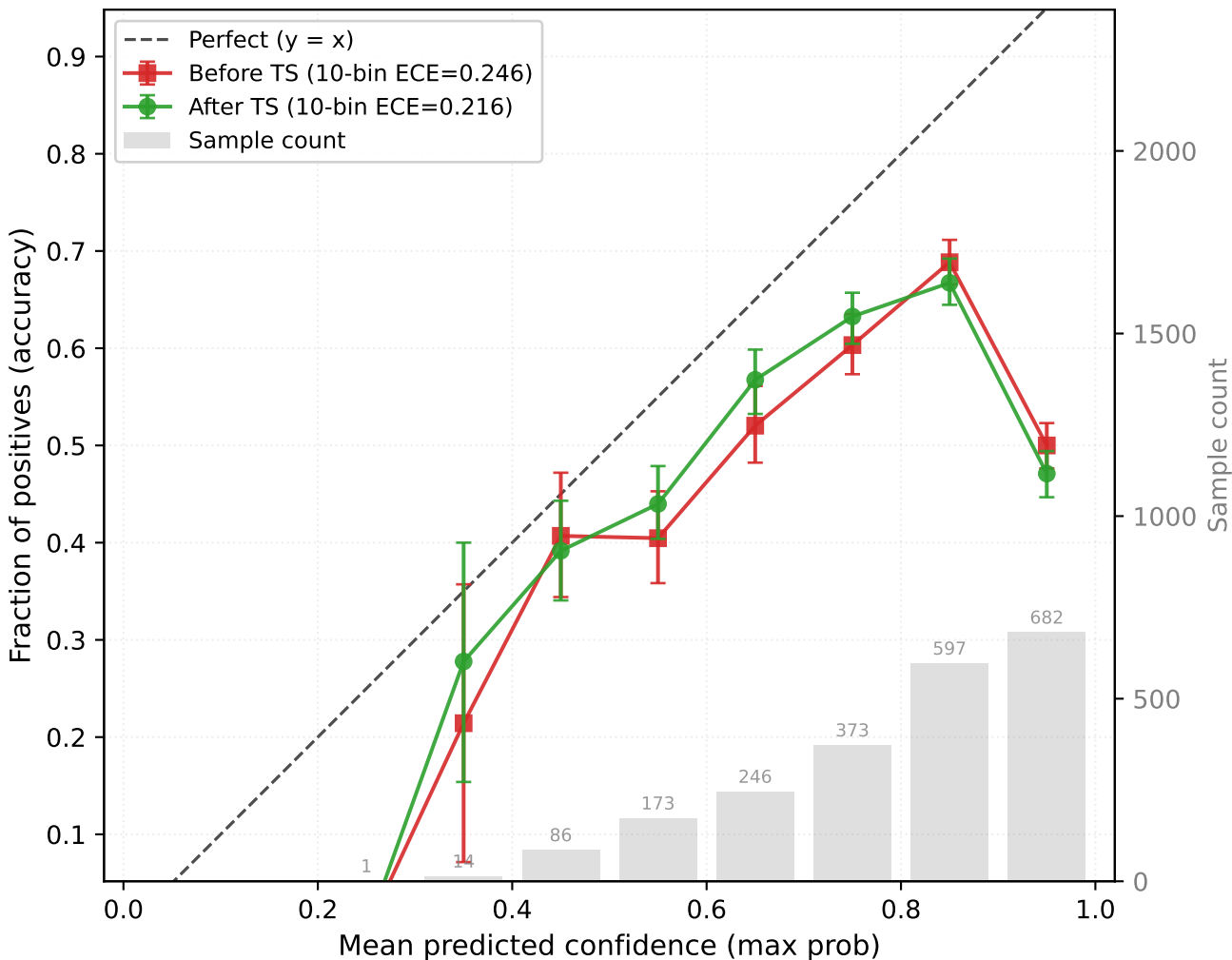
CHAPMAN → PTBXL (resnet1d, seed42) OOD target-test (n=2172, T=1.125)
