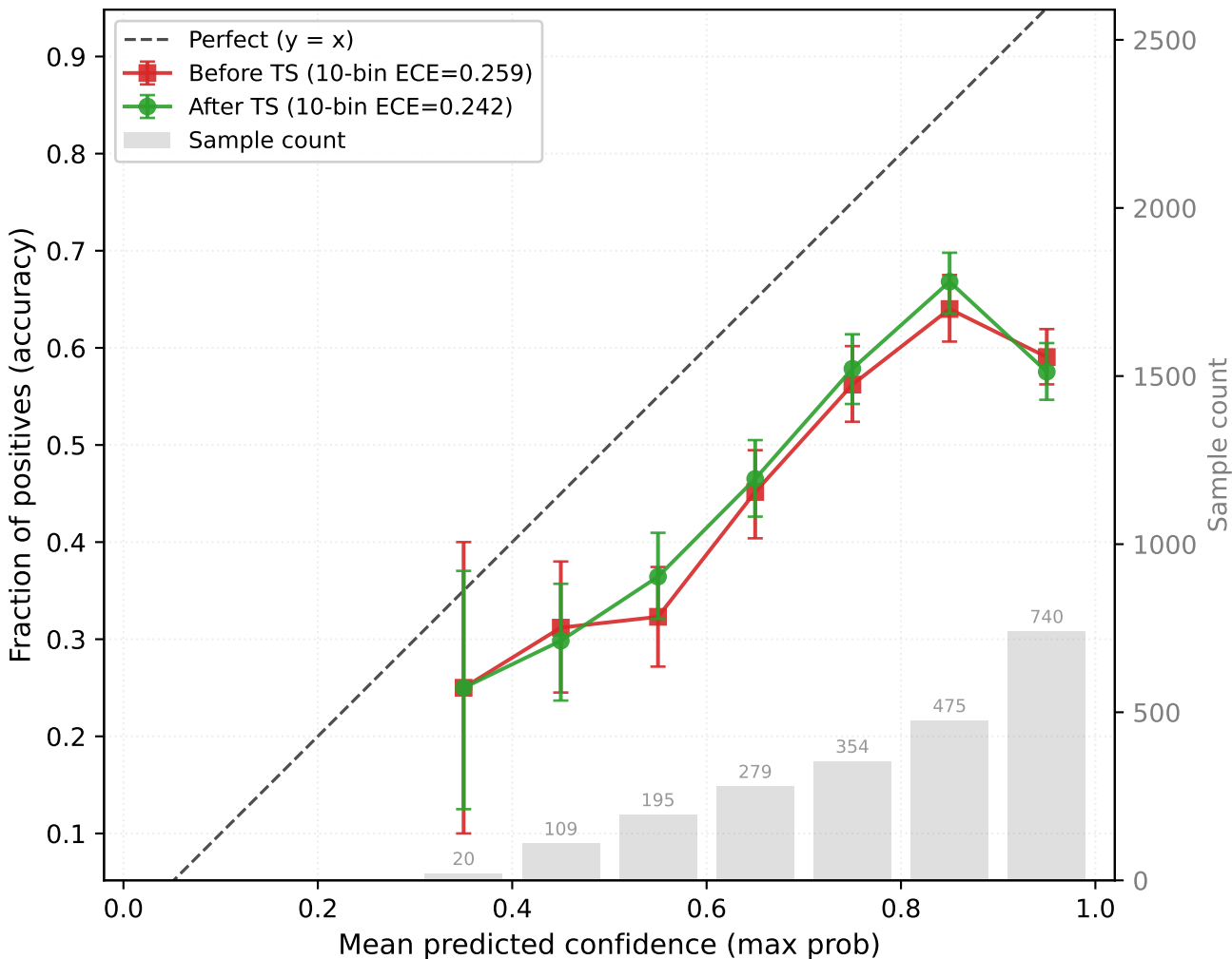
CHAPMAN → PTBXL (resnet1d, seed44) OOD target-test (n=2172, T=1.068)
