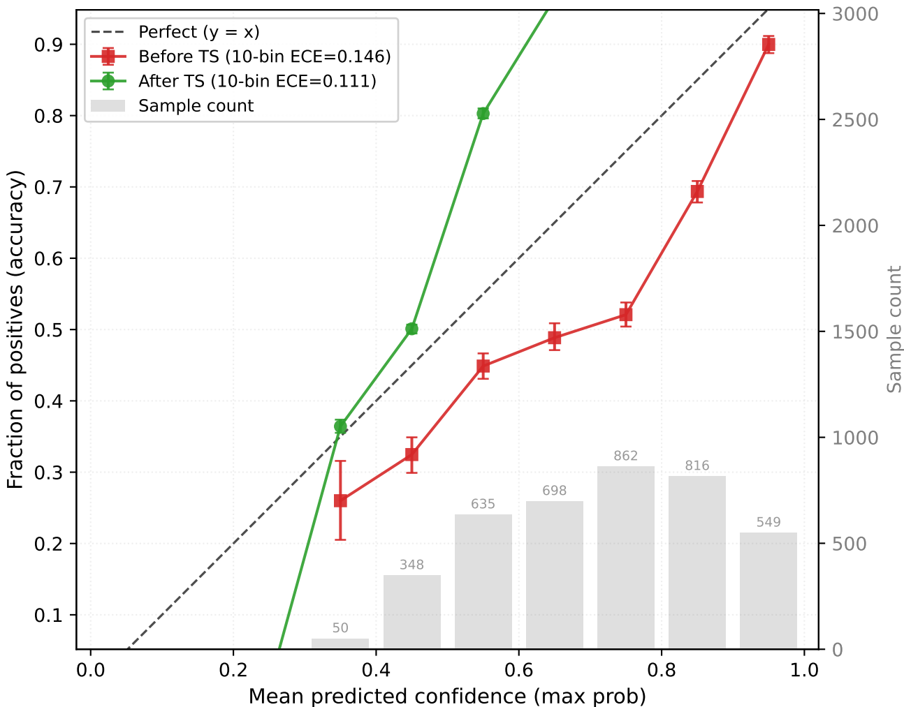
CPSC → CHAPMAN (inceptiontime, seed43) OOD target-test (n=3958, T=2.821)
