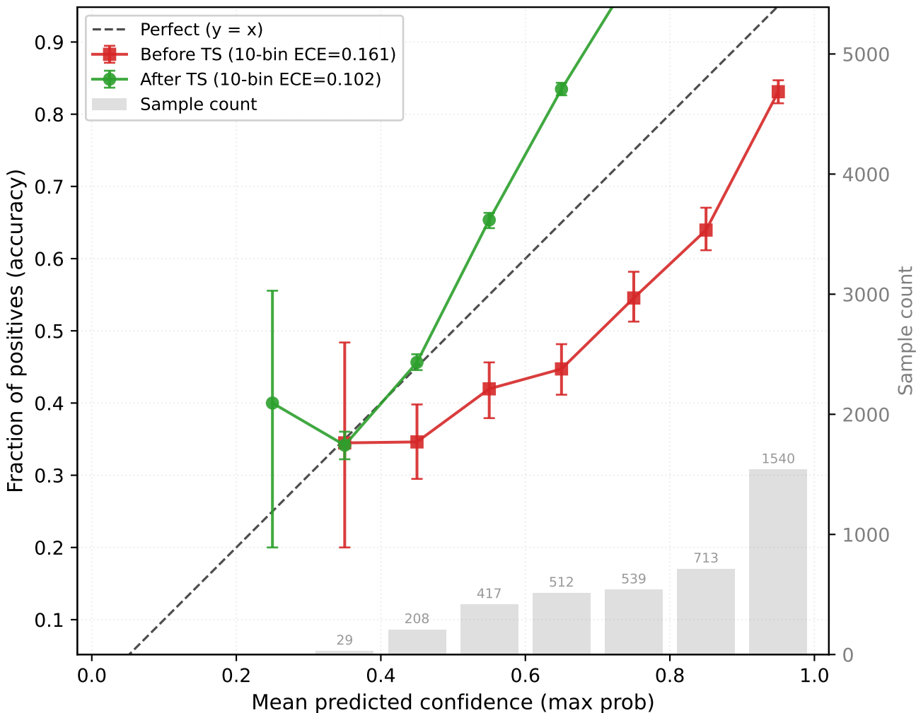
CPSC → CHAPMAN (resnet1d, seed43) OOD target-test (n=3958, T=2.551)
