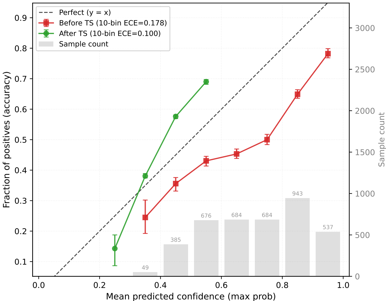
CPSC → CHAPMAN (resnet1d, seed44) OOD target-test (n=3958, T=3.129)
