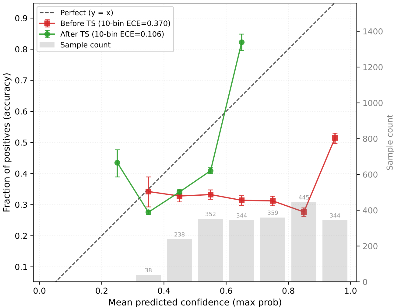
CPSC \rightarrow PTBXL (resnet1d, seed45) OOD target-test (n=2120, T=3.124)
