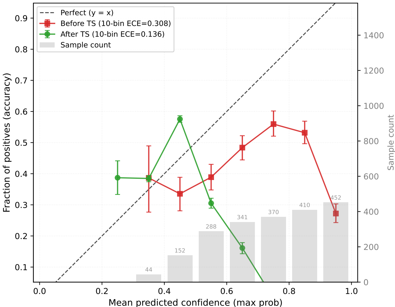
PTBXL \rightarrow CPSC (inceptiontime, seed45) OOD target-test (n=2057, T=3.409)
