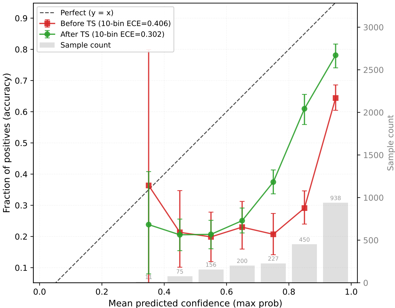
CHAPMAN → CPSC (inceptiontime, seed44) OOD target-test (n=2057, T=1.612)
