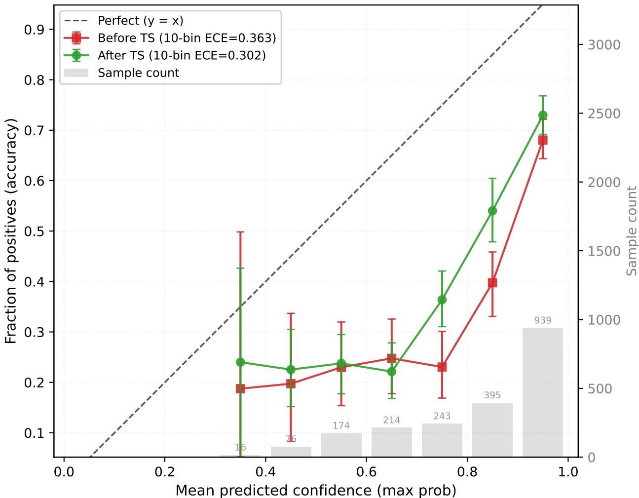
CHAPMAN → CPSC (resnet1d, seed44) OOD target-test (n=2057, T=1.324)
