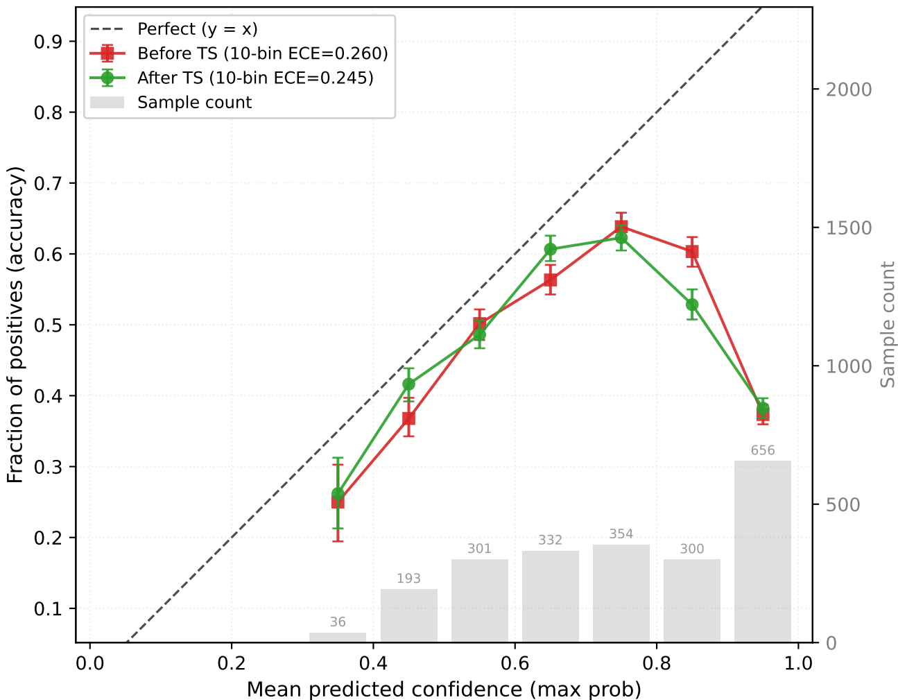
CHAPMAN → PTBXL (inceptiontime, seed44) OOD target-test (n=2172, T=1.059)
