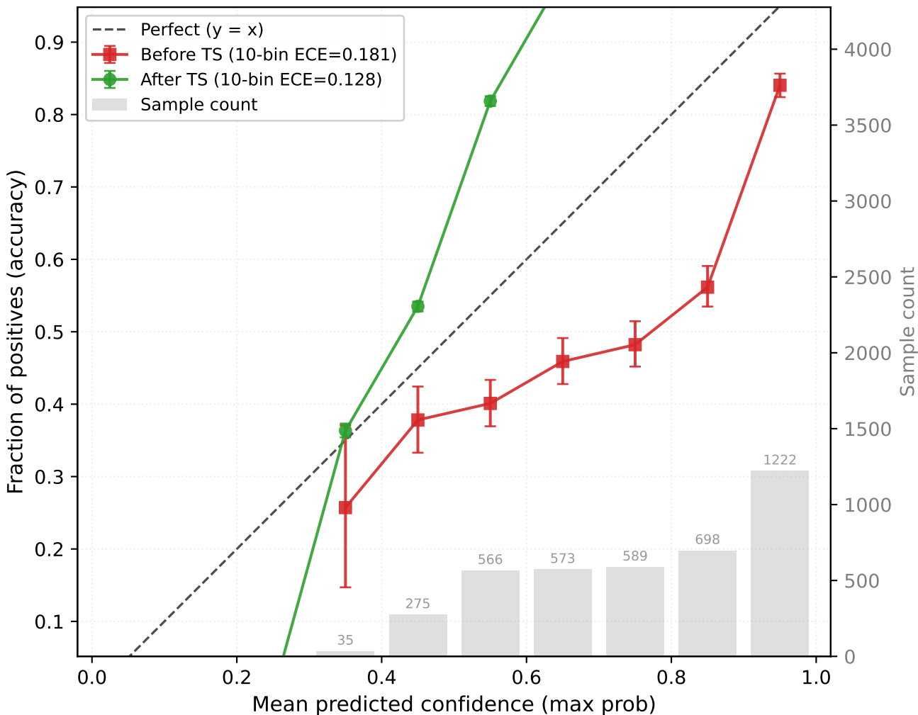
CPSC → CHAPMAN (inceptiontime, seed45) OOD target-test (n=3958, T=3.438)
