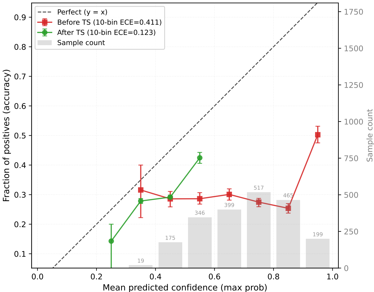
CPSC \rightarrow PTBXL (resnet1d, seed44) OOD target-test (n=2120, T=3.250)
