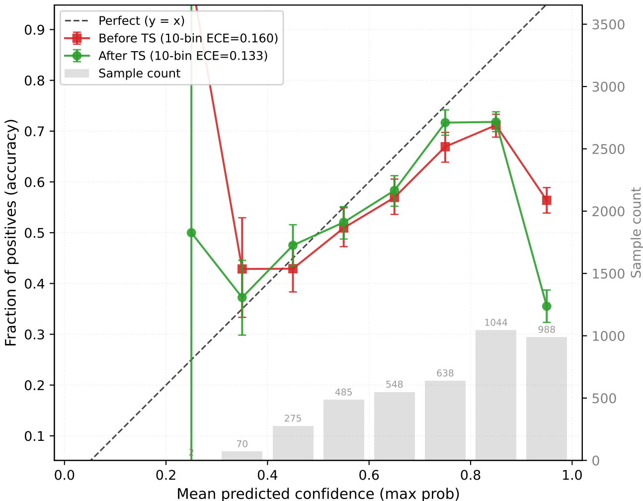
PTBXL → CHAPMAN (inceptiontime, seed43) OOD target-test (n=4050, T=1.106)
