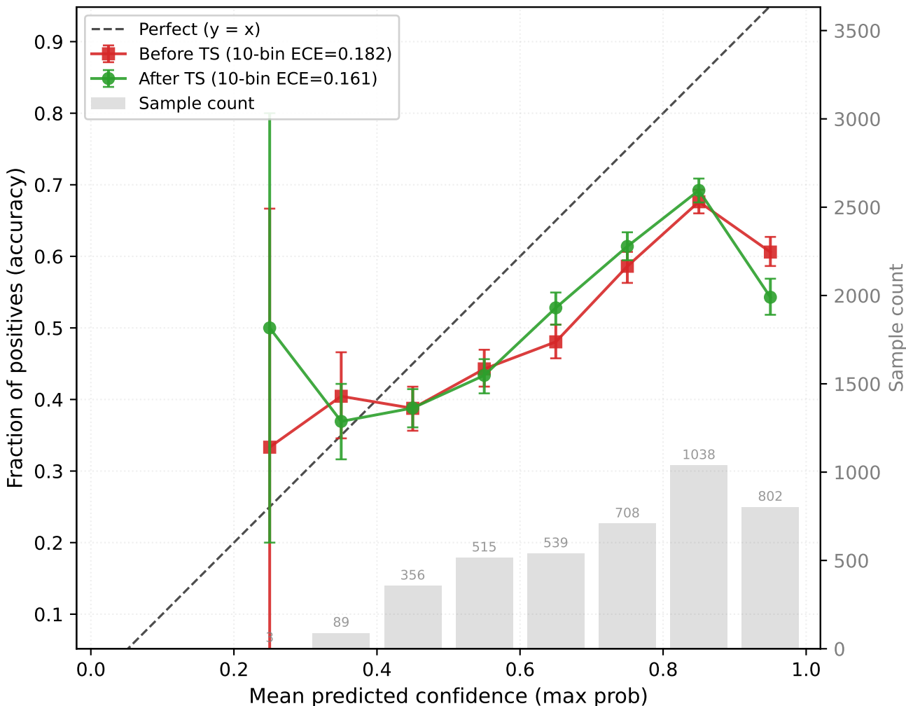
PTBXL → CHAPMAN (inceptiontime, seed44) OOD target-test (n=4050, T=1.074)
