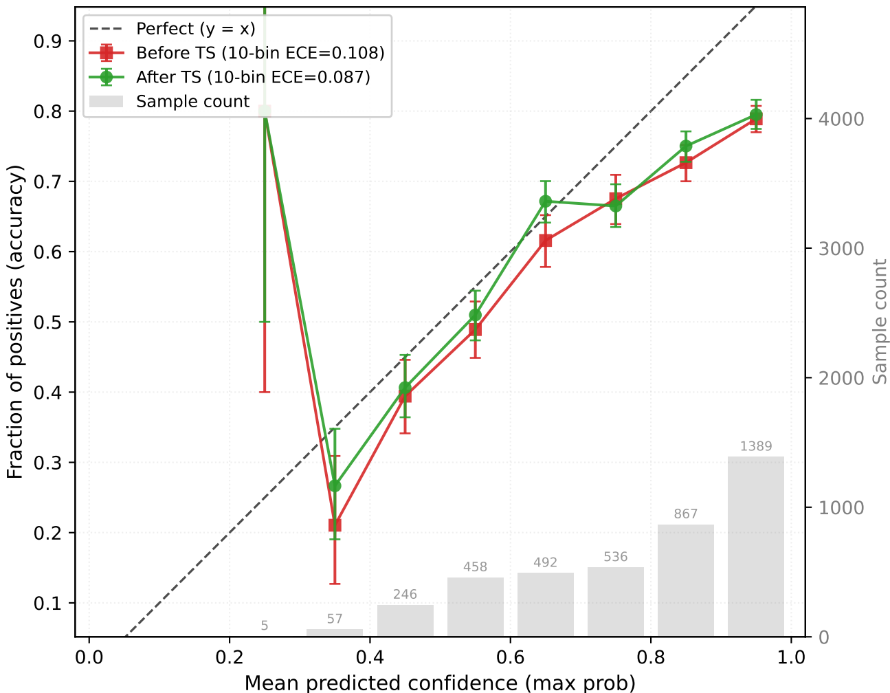
PTBXL \rightarrow CHAPMAN (resnet1d, seed42) OOD target-test (n=4050, T=1.108)
