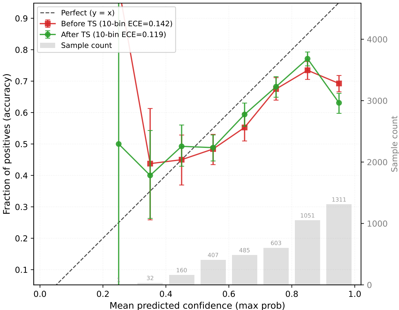
PTBXL \rightarrow CHAPMAN (resnet1d, seed44) OOD target-test (n=4050, T=1.103)
