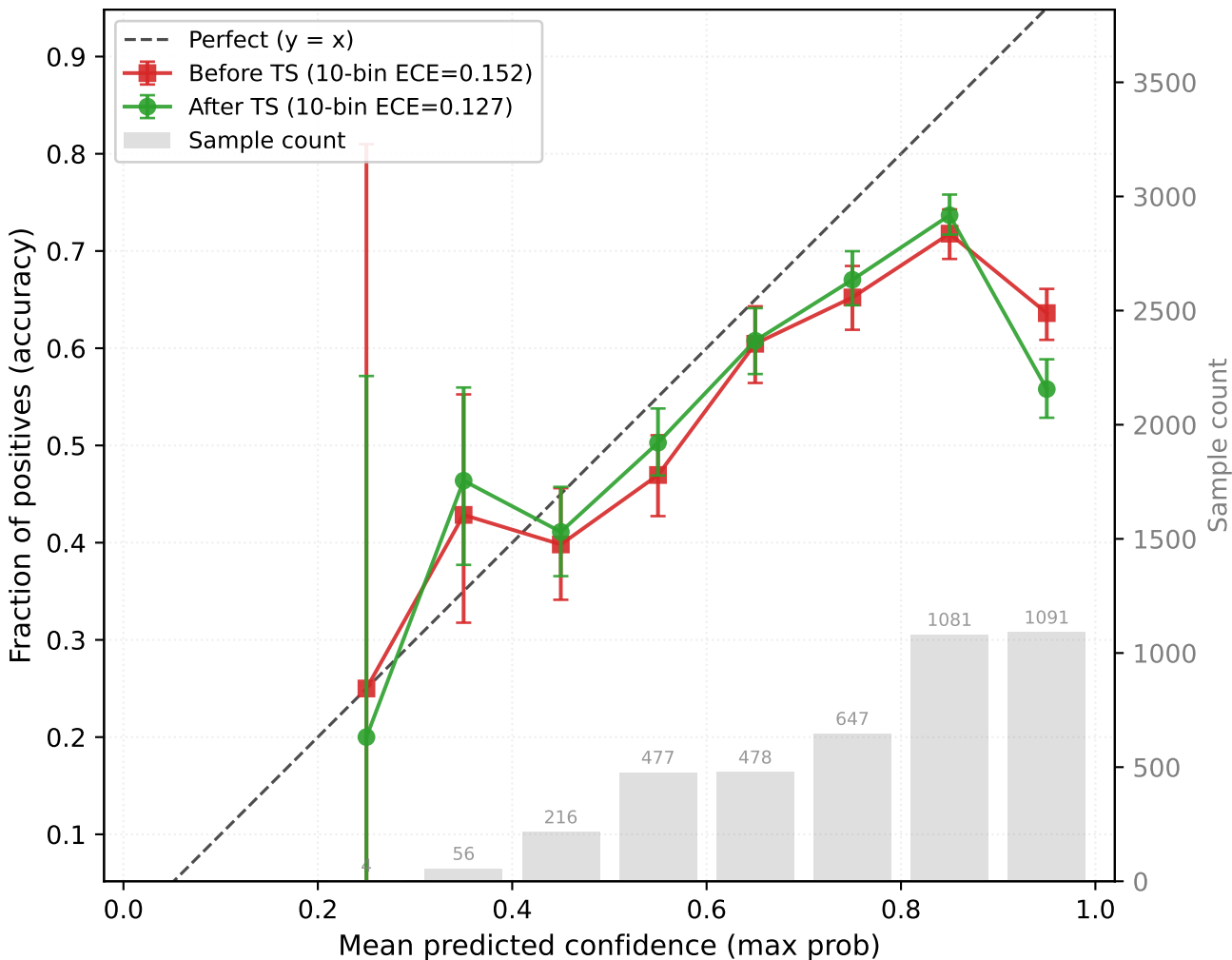
PTBXL \rightarrow CHAPMAN (resnet1d, seed45) OOD target-test (n=4050, T=1.107)
